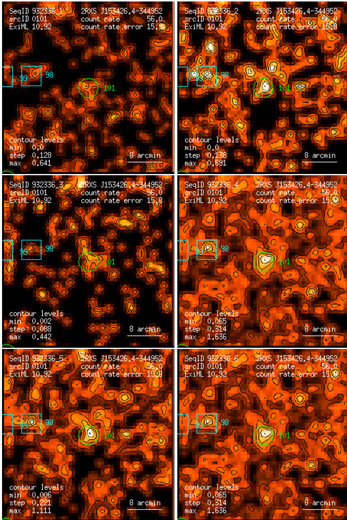
Figure 101: RASS 932336: detection 0101: band rate images, Gaussian filter: (1) PSPC channels 11 – 41, (2) 52 – 90, (3) 91 – 201, (4) 11 – 235, (5) 52 – 201, (6) 11 – 201. Broad band rates in counts/ks. Band rate contour levels in counts/ks/arcmin 2 .
