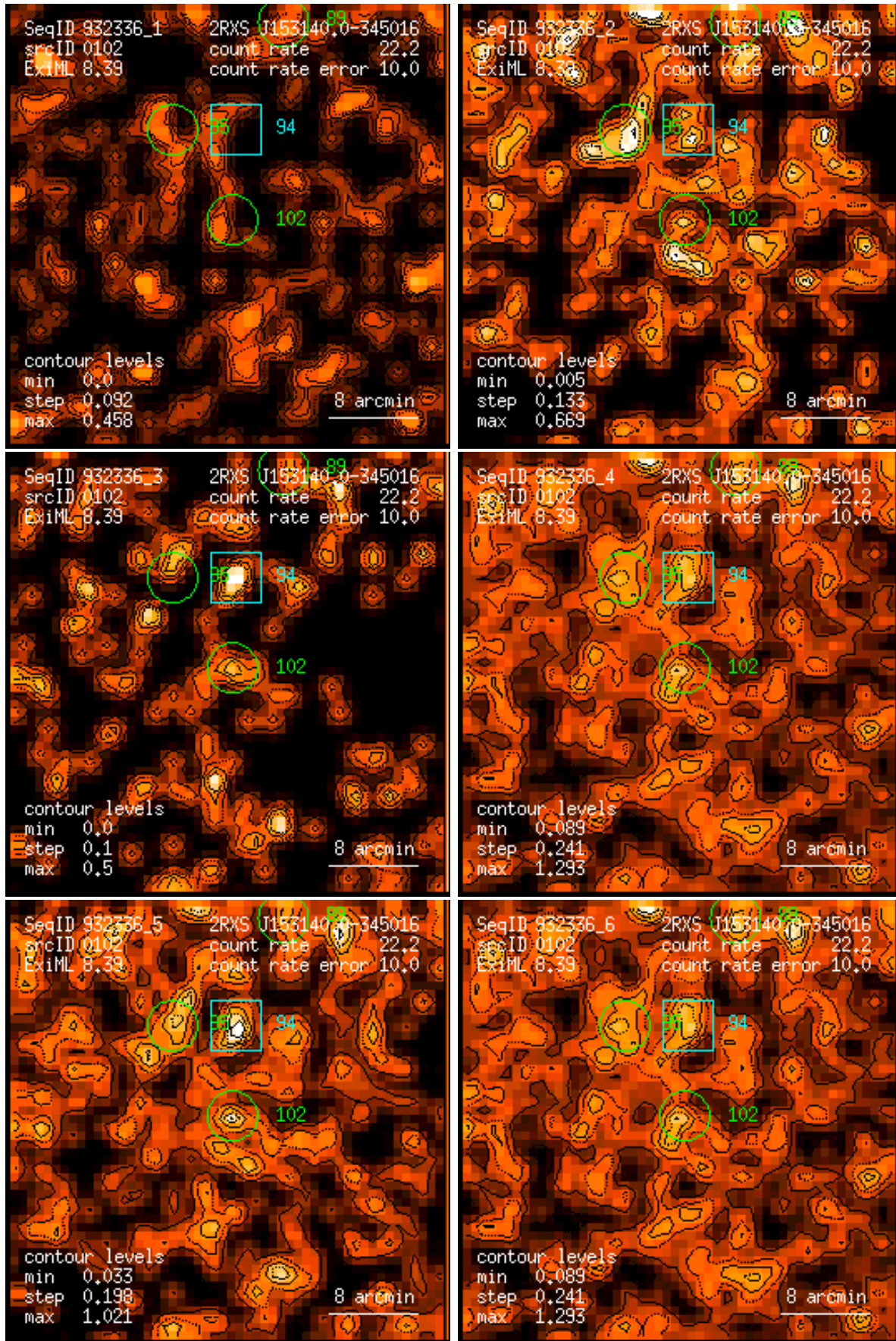
Figure 102: RASS 932336: detection 0102: band rate images, Gaussian filter: (1) PSPC channels 11 – 41, (2) 52 – 90, (3) 91 – 201, (4) 11 – 235, (5) 52 – 201, (6) 11 – 201. Broad band rates in counts/ks. Band rate contour levels in counts/ks/arcmin 2 .
