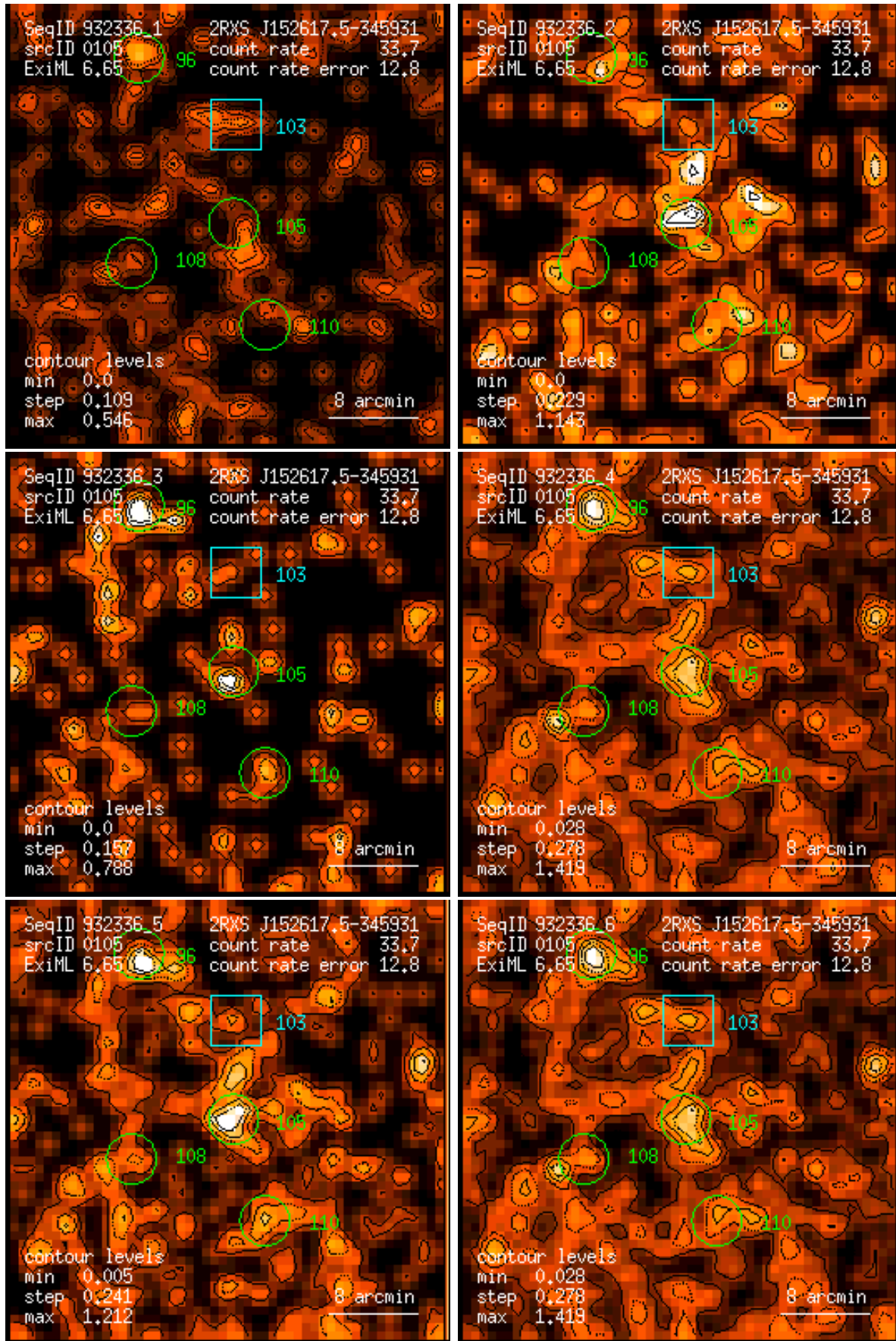
Figure 105: RASS 932336: detection 0105: band rate images, Gaussian filter: (1) PSPC channels 11 – 41, (2) 52 – 90, (3) 91 – 201, (4) 11 – 235, (5) 52 – 201, (6) 11 – 201. Broad band rates in counts/ks. Band rate contour levels in counts/ks/arcmin 2 .
