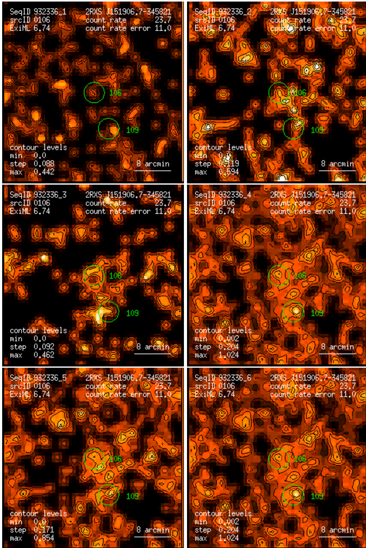
Figure 106: RASS 932336: detection 0106: band rate images, Gaussian filter: (1) PSPC channels 11 – 41, (2) 52 – 90, (3) 91 – 201, (4) 11 – 235, (5) 52 – 201, (6) 11 – 201. Broad band rates in counts/ks. Band rate contour levels in counts/ks/arcmin 2 .
