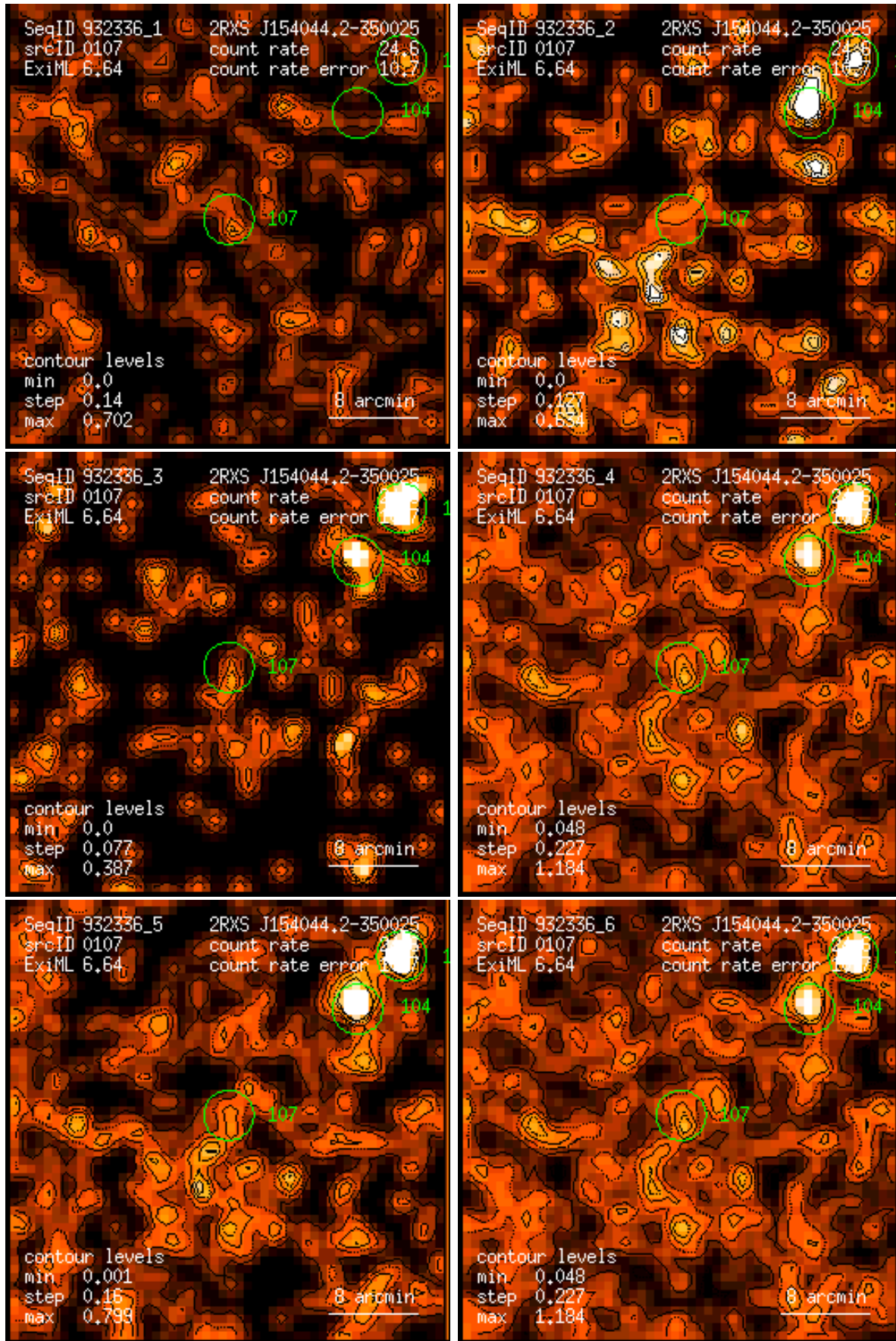
Figure 107: RASS 932336: detection 0107: band rate images, Gaussian filter: (1) PSPC channels 11 – 41, (2) 52 – 90, (3) 91 – 201, (4) 11 – 235, (5) 52 – 201, (6) 11 – 201. Broad band rates in counts/ks. Band rate contour levels in counts/ks/arcmin 2 .
