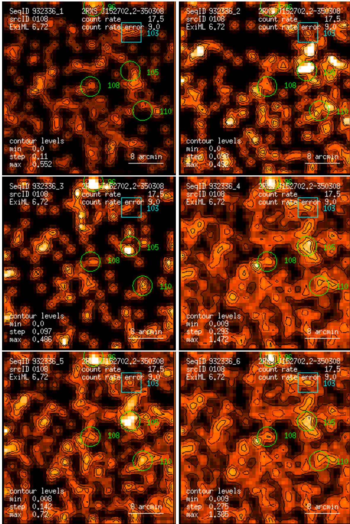
Figure 108: RASS 932336: detection 0108: band rate images, Gaussian filter: (1) PSPC channels 11 – 41, (2) 52 – 90, (3) 91 – 201, (4) 11 – 235, (5) 52 – 201, (6) 11 – 201. Broad band rates in counts/ks. Band rate contour levels in counts/ks/arcmin 2 .
