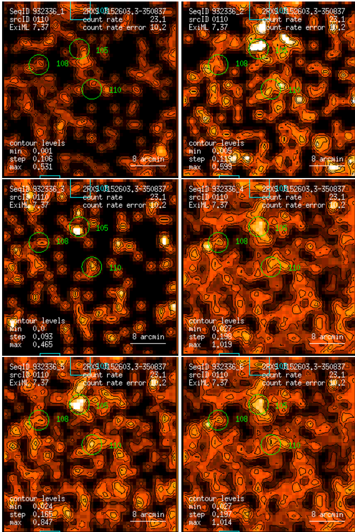
Figure 110: RASS 932336: detection 0110: band rate images, Gaussian filter: (1) PSPC channels 11 – 41, (2) 52 – 90, (3) 91 – 201, (4) 11 – 235, (5) 52 – 201, (6) 11 – 201. Broad band rates in counts/ks. Band rate contour levels in counts/ks/arcmin 2 .
