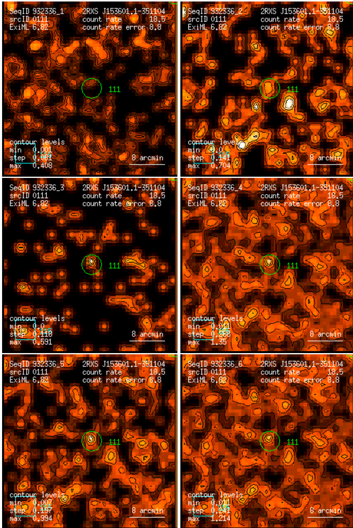
Figure 111: RASS 932336: detection 0111: band rate images, Gaussian filter: (1) PSPC channels 11 – 41, (2) 52 – 90, (3) 91 – 201, (4) 11 – 235, (5) 52 – 201, (6) 11 – 201. Broad band rates in counts/ks. Band rate contour levels in counts/ks/arcmin 2 .
