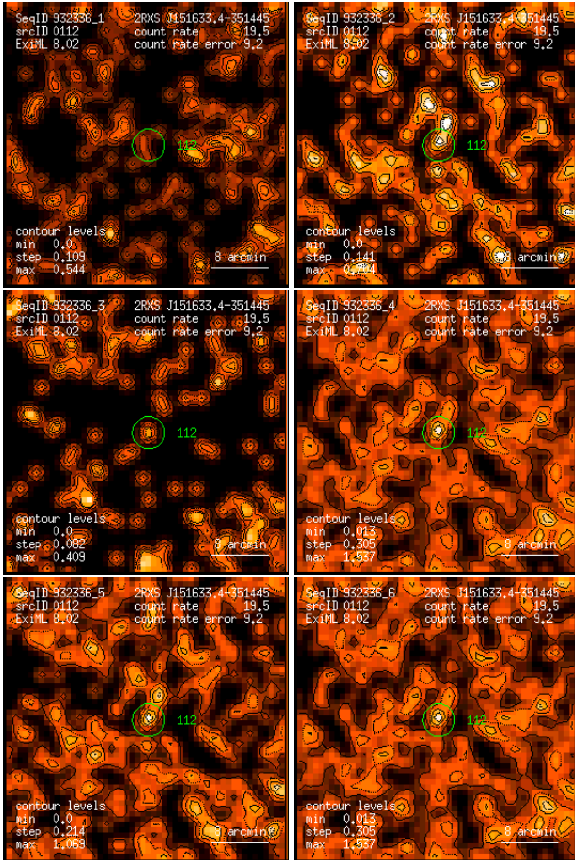
Figure 112: RASS 932336: detection 0112: band rate images, Gaussian filter: (1) PSPC channels 11 – 41, (2) 52 – 90, (3) 91 – 201, (4) 11 – 235, (5) 52 – 201, (6) 11 – 201. Broad band rates in counts/ks. Band rate contour levels in counts/ks/arcmin 2 .
