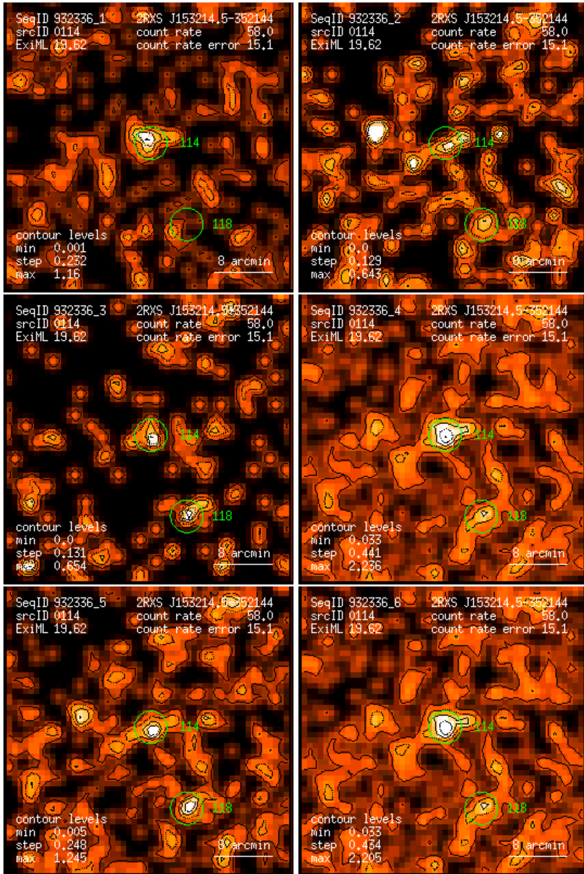
Figure 114: RASS 932336: detection 0114: band rate images, Gaussian filter: (1) PSPC channels 11 – 41, (2) 52 – 90, (3) 91 – 201, (4) 11 – 235, (5) 52 – 201, (6) 11 – 201. Broad band rates in counts/ks. Band rate contour levels in counts/ks/arcmin 2 .
