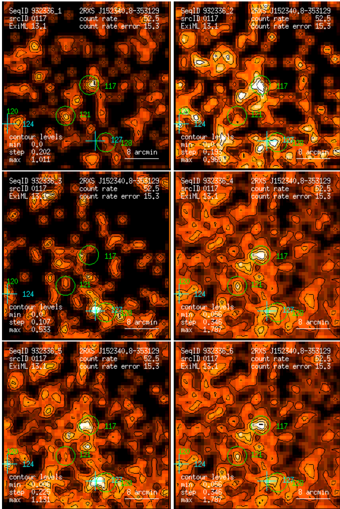
Figure 117: RASS 932336: detection 0117: band rate images, Gaussian filter: (1) PSPC channels 11 – 41, (2) 52 – 90, (3) 91 – 201, (4) 11 – 235, (5) 52 – 201, (6) 11 – 201. Broad band rates in counts/ks. Band rate contour levels in counts/ks/arcmin 2 .
