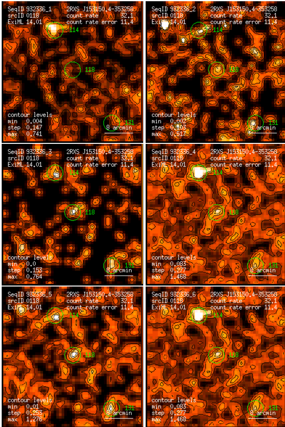
Figure 118: RASS 932336: detection 0118: band rate images, Gaussian filter: (1) PSPC channels 11 – 41, (2) 52 – 90, (3) 91 – 201, (4) 11 – 235, (5) 52 – 201, (6) 11 – 201. Broad band rates in counts/ks. Band rate contour levels in counts/ks/arcmin 2 .
