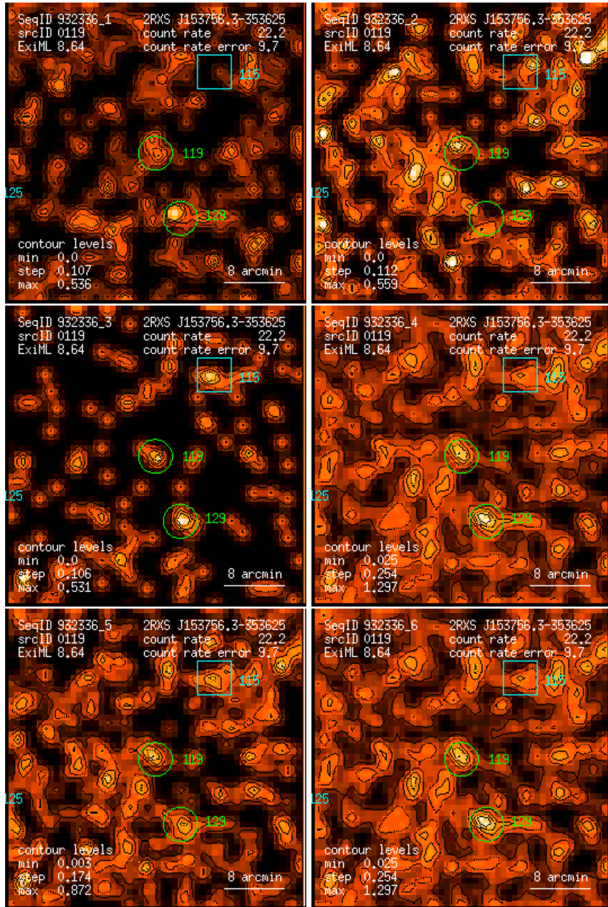
Figure 119: RASS 932336: detection 0119: band rate images, Gaussian filter: (1) PSPC channels 11 – 41, (2) 52 – 90, (3) 91 – 201, (4) 11 – 235, (5) 52 – 201, (6) 11 – 201. Broad band rates in counts/ks. Band rate contour levels in counts/ks/arcmin 2 .
