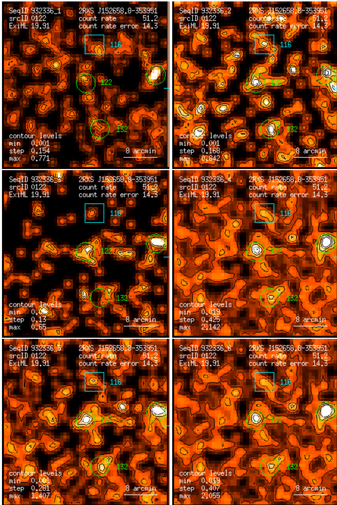
Figure 122: RASS 932336: detection 0122: band rate images, Gaussian filter: (1) PSPC channels 11 – 41, (2) 52 – 90, (3) 91 – 201, (4) 11 – 235, (5) 52 – 201, (6) 11 – 201. Broad band rates in counts/ks. Band rate contour levels in counts/ks/arcmin 2 .
