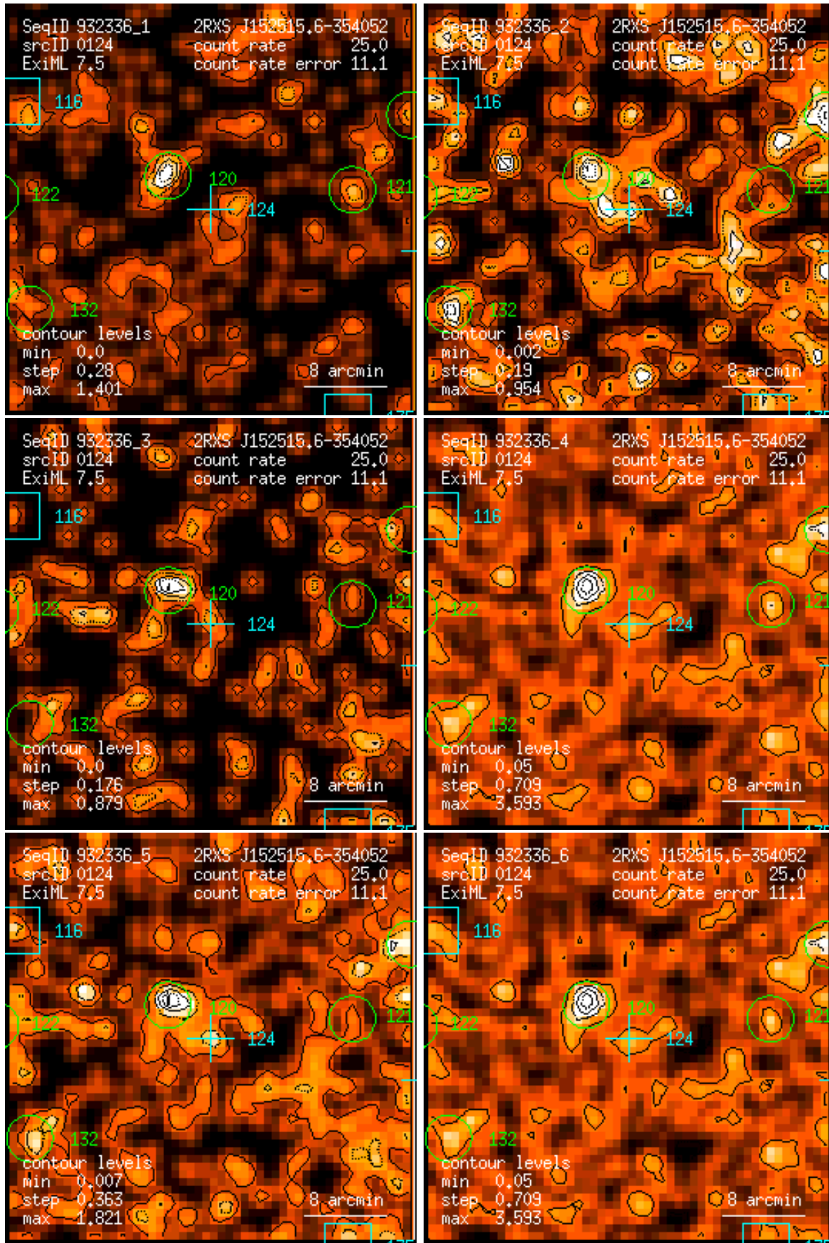
Figure 124: RASS 932336: detection 0124: band rate images, Gaussian filter: (1) PSPC channels 11 – 41, (2) 52 – 90, (3) 91 – 201, (4) 11 – 235, (5) 52 – 201, (6) 11 – 201. Broad band rates in counts/ks. Band rate contour levels in counts/ks/arcmin 2 .
