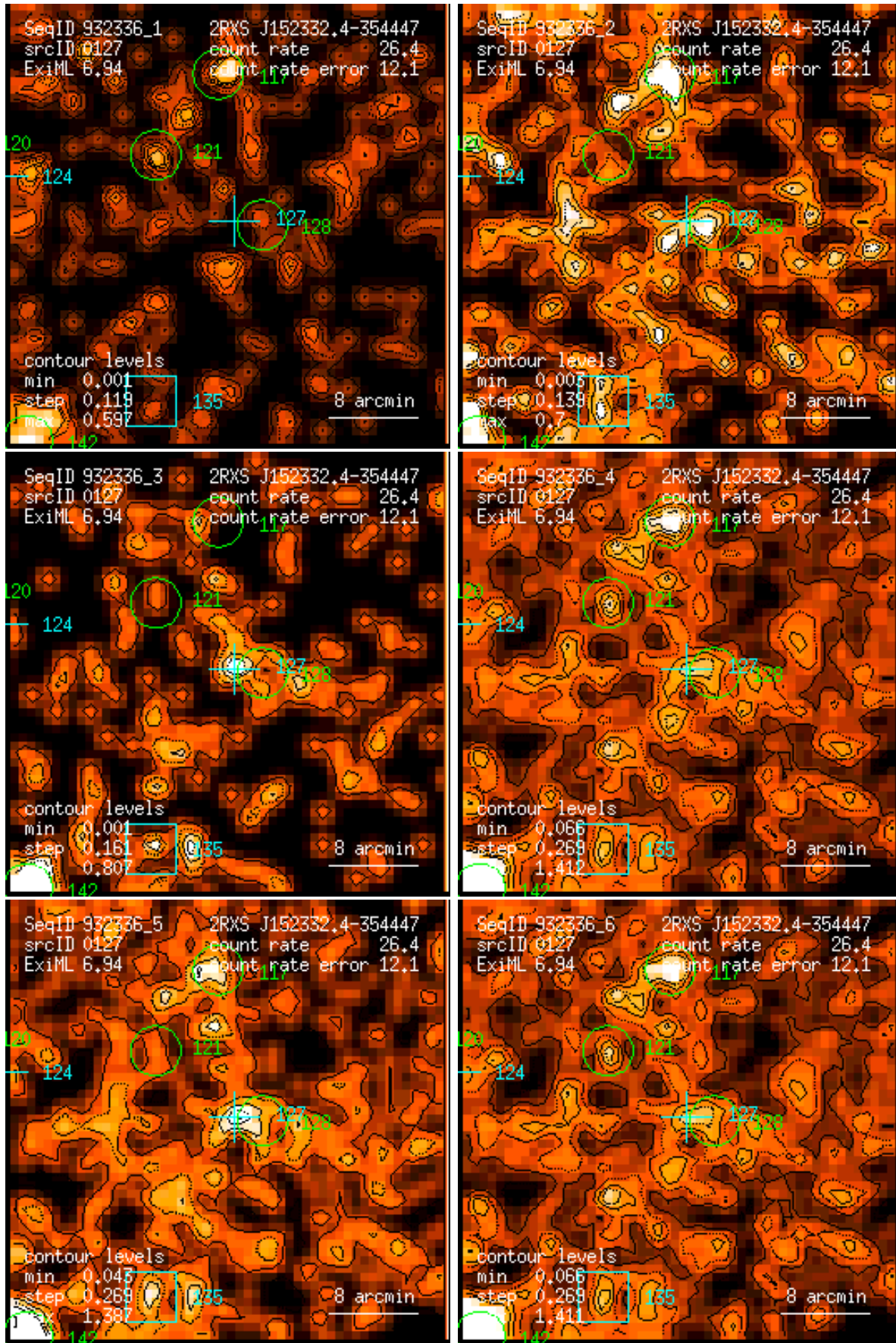
Figure 127: RASS 932336: detection 0127: band rate images, Gaussian filter: (1) PSPC channels 11 – 41, (2) 52 – 90, (3) 91 – 201, (4) 11 – 235, (5) 52 – 201, (6) 11 – 201. Broad band rates in counts/ks. Band rate contour levels in counts/ks/arcmin 2 .
