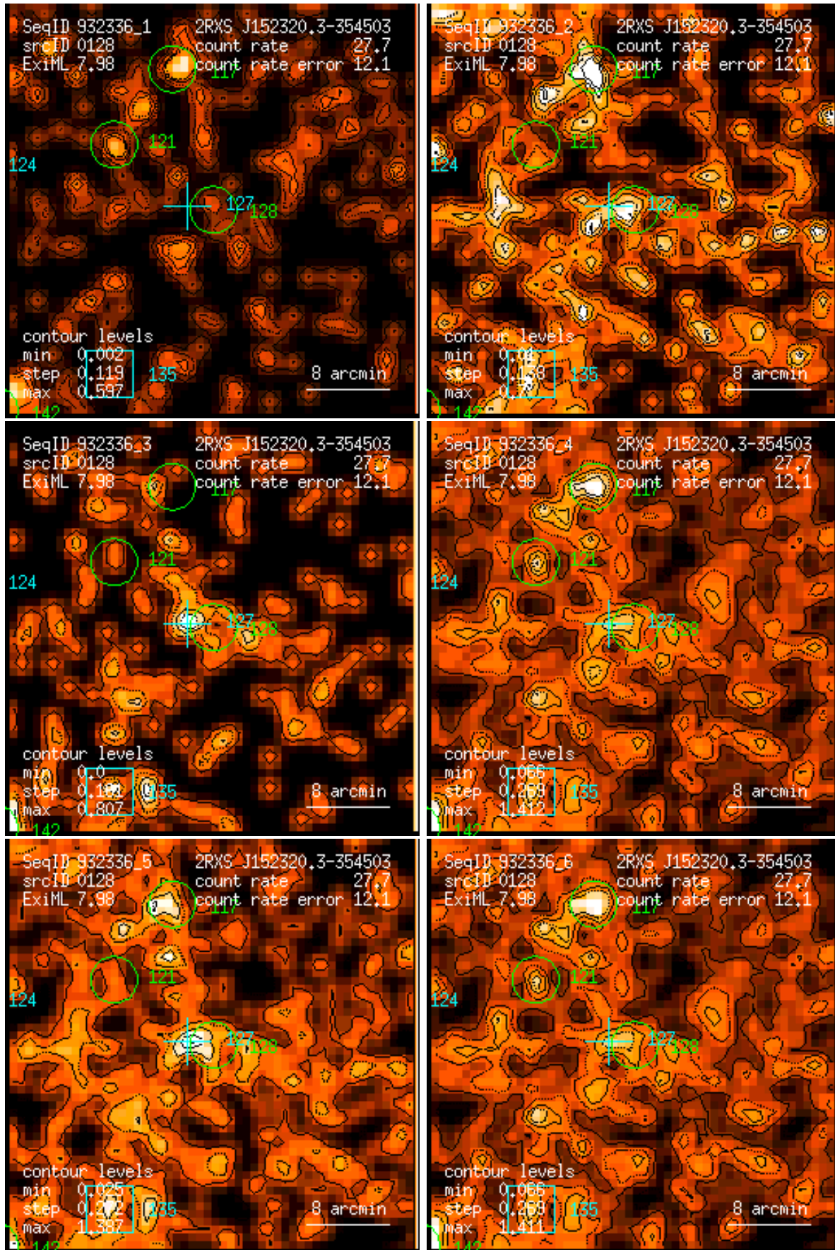
Figure 128: RASS 932336: detection 0128: band rate images, Gaussian filter: (1) PSPC channels 11 – 41, (2) 52 – 90, (3) 91 – 201, (4) 11 – 235, (5) 52 – 201, (6) 11 – 201. Broad band rates in counts/ks. Band rate contour levels in counts/ks/arcmin 2 .
