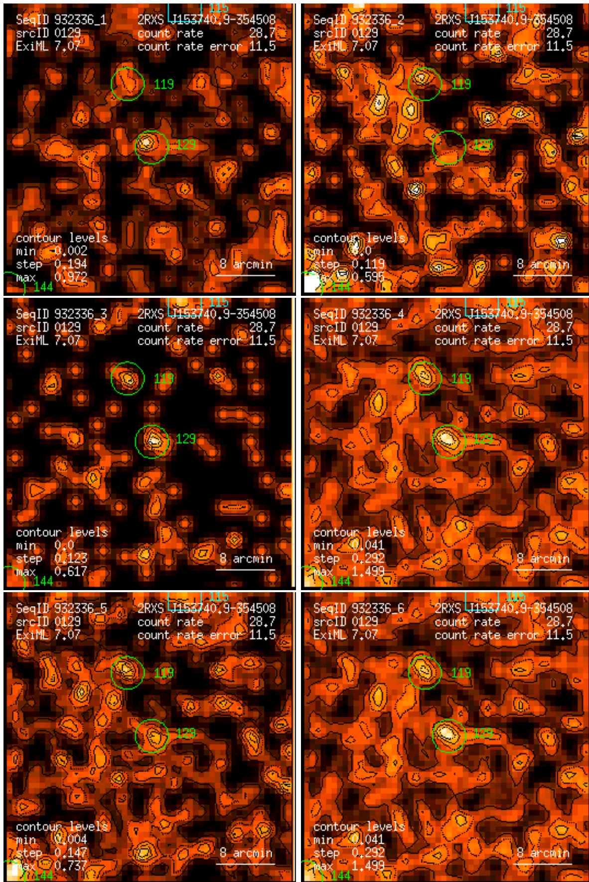
Figure 129: RASS 932336: detection 0129: band rate images, Gaussian filter: (1) PSPC channels 11 – 41, (2) 52 – 90, (3) 91 – 201, (4) 11 – 235, (5) 52 – 201, (6) 11 – 201. Broad band rates in counts/ks. Band rate contour levels in counts/ks/arcmin 2 .
