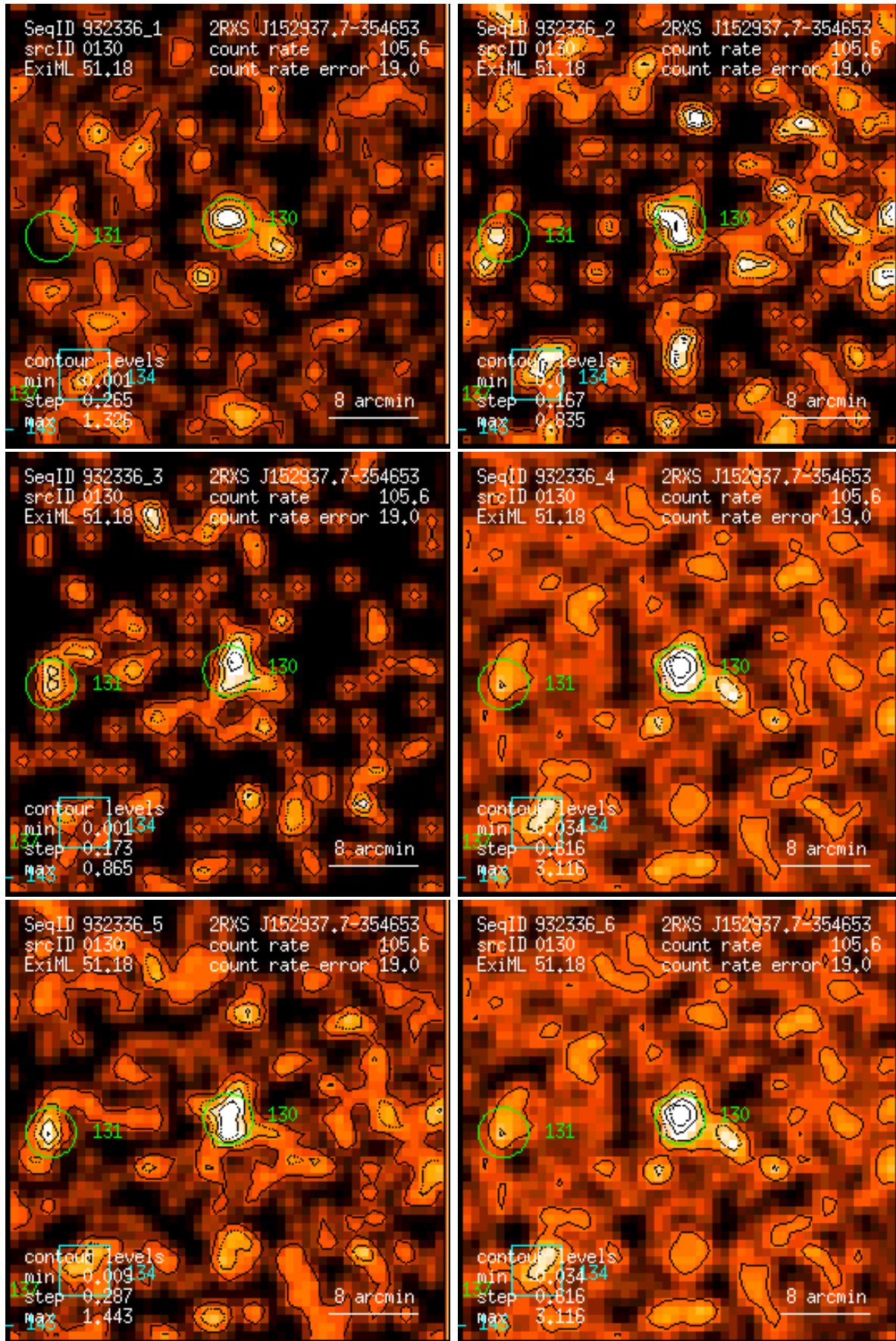
Figure 130: RASS 932336: detection 0130: band rate images, Gaussian filter: (1) PSPC channels 11 – 41, (2) 52 – 90, (3) 91 – 201, (4) 11 – 235, (5) 52 – 201, (6) 11 – 201. Broad band rates in counts/ks. Band rate contour levels in counts/ks/arcmin 2 .
