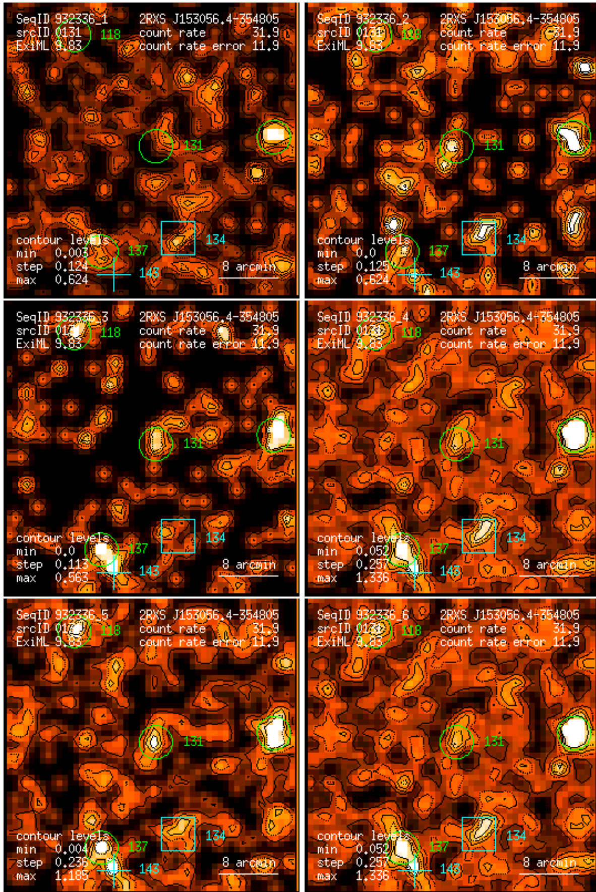
Figure 131: RASS 932336: detection 0131: band rate images, Gaussian filter: (1) PSPC channels 11 – 41, (2) 52 – 90, (3) 91 – 201, (4) 11 – 235, (5) 52 – 201, (6) 11 – 201. Broad band rates in counts/ks. Band rate contour levels in counts/ks/arcmin 2 .
