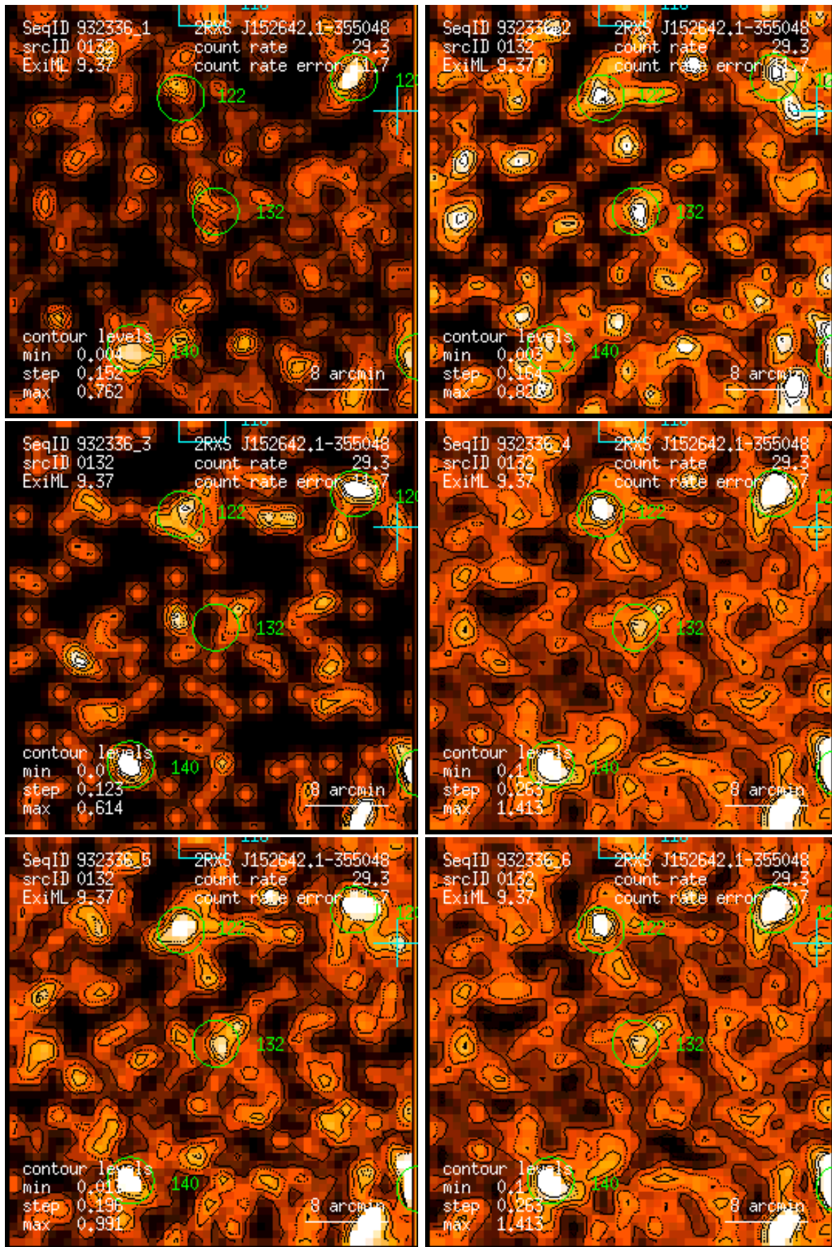
Figure 132: RASS 932336: detection 0132: band rate images, Gaussian filter: (1) PSPC channels 11 – 41, (2) 52 – 90, (3) 91 – 201, (4) 11 – 235, (5) 52 – 201, (6) 11 – 201. Broad band rates in counts/ks. Band rate contour levels in counts/ks/arcmin 2 .
