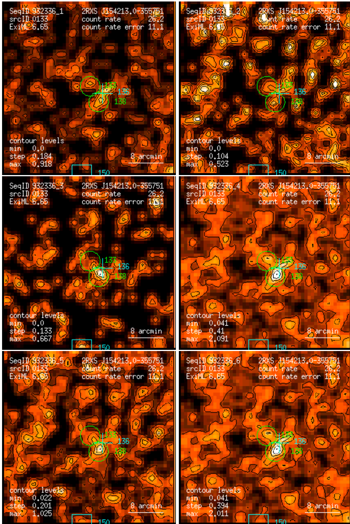
Figure 133: RASS 932336: detection 0133: band rate images, Gaussian filter: (1) PSPC channels 11 – 41, (2) 52 – 90, (3) 91 – 201, (4) 11 – 235, (5) 52 – 201, (6) 11 – 201. Broad band rates in counts/ks. Band rate contour levels in counts/ks/arcmin 2 .
