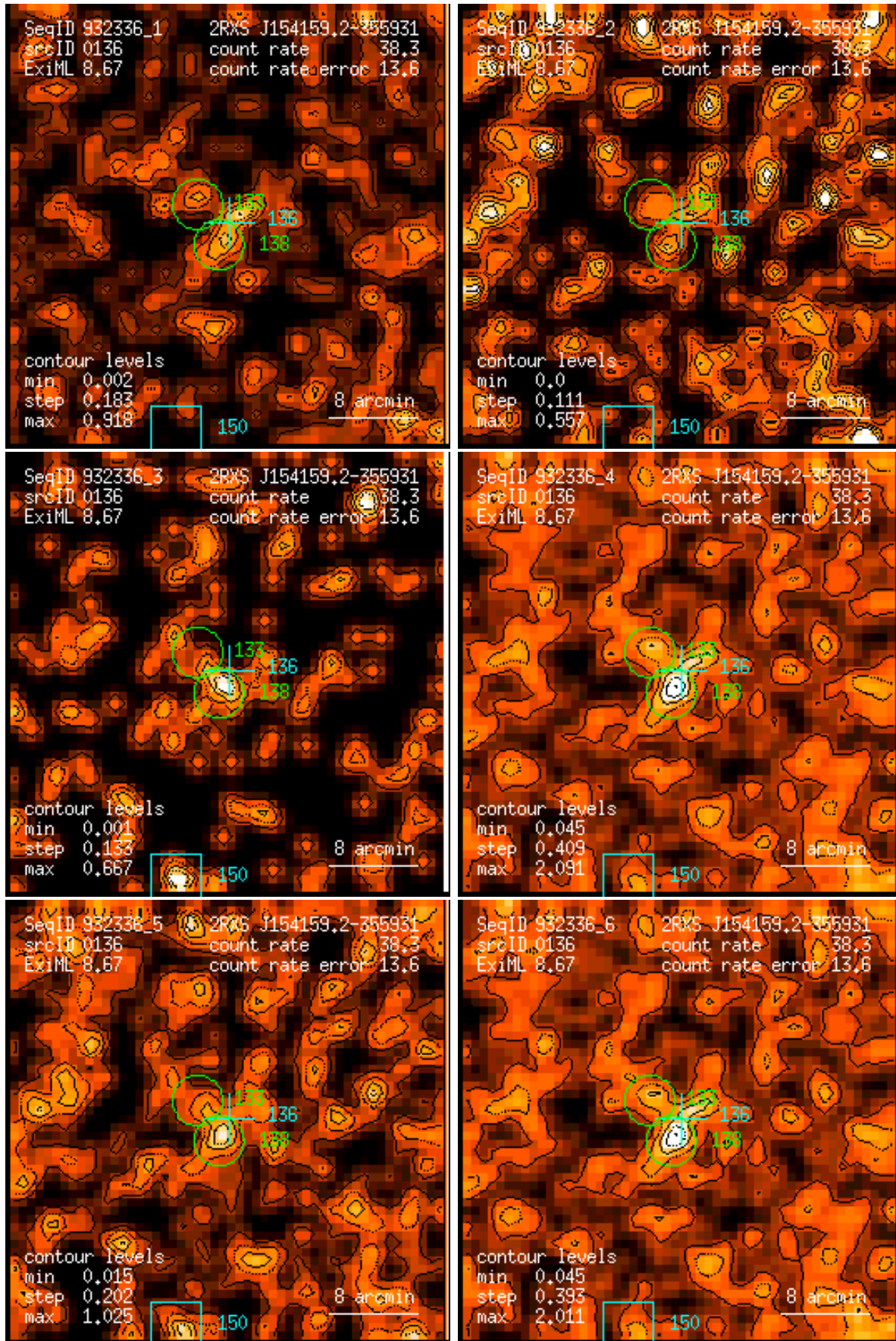
Figure 136: RASS 932336: detection 0136: band rate images, Gaussian filter: (1) PSPC channels 11 – 41, (2) 52 – 90, (3) 91 – 201, (4) 11 – 235, (5) 52 – 201, (6) 11 – 201. Broad band rates in counts/ks. Band rate contour levels in counts/ks/arcmin 2 .
