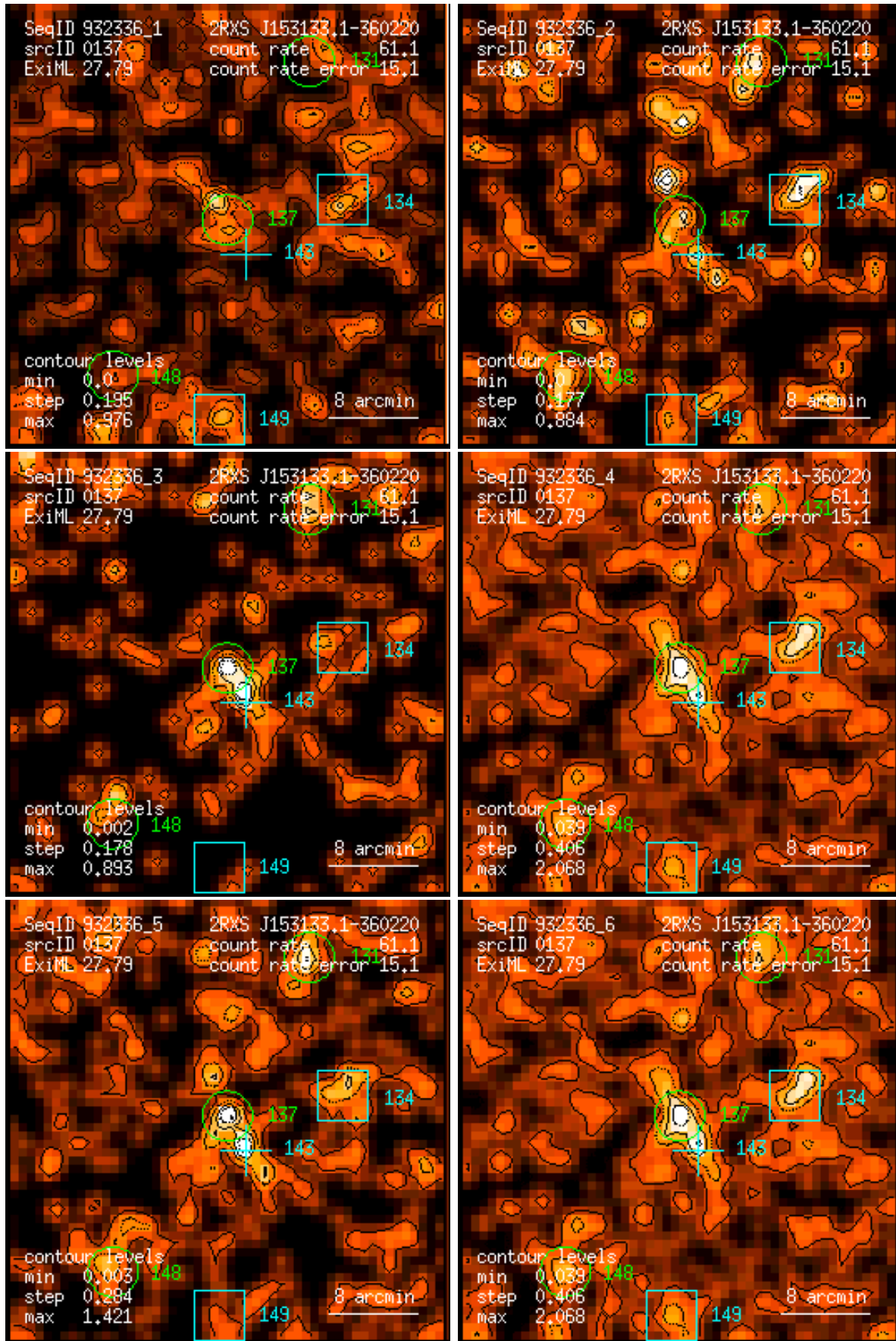
Figure 137: RASS 932336: detection 0137: band rate images, Gaussian filter: (1) PSPC channels 11 – 41, (2) 52 – 90, (3) 91 – 201, (4) 11 – 235, (5) 52 – 201, (6) 11 – 201. Broad band rates in counts/ks. Band rate contour levels in counts/ks/arcmin 2 .
