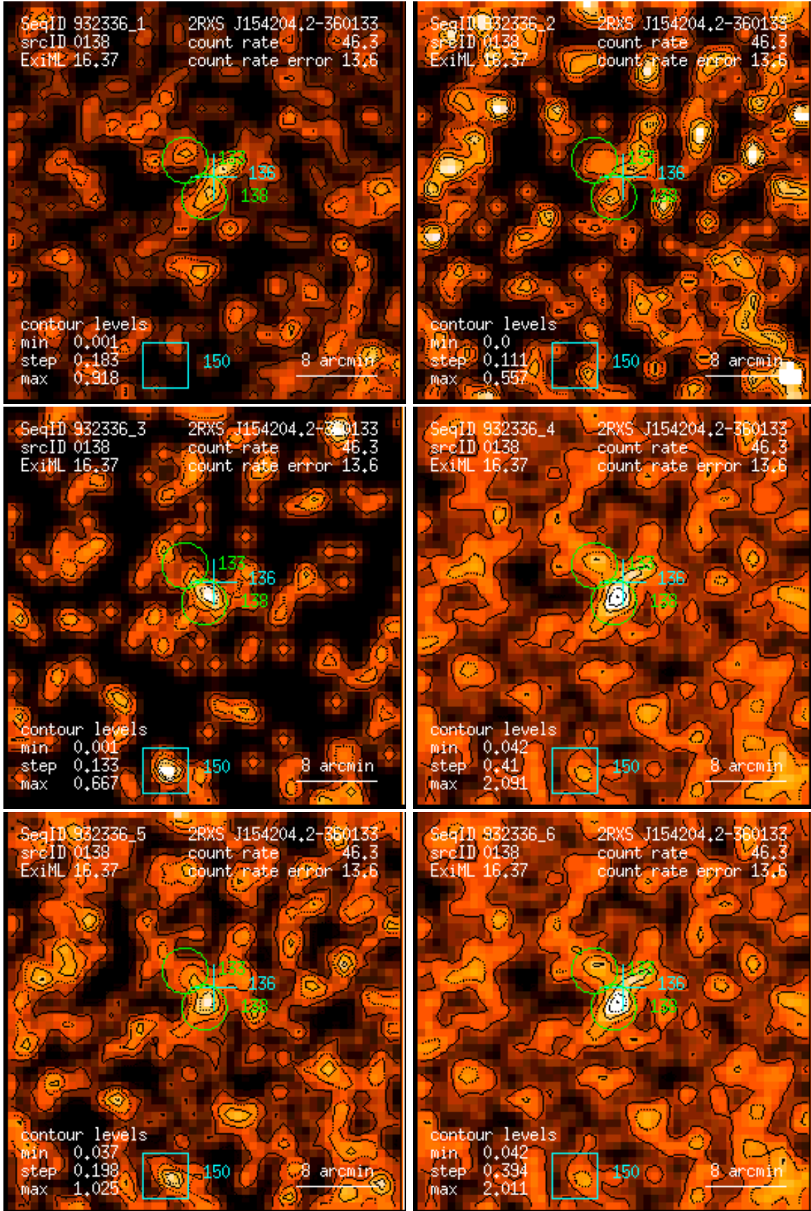
Figure 138: RASS 932336: detection 0138: band rate images, Gaussian filter: (1) PSPC channels 11 – 41, (2) 52 – 90, (3) 91 – 201, (4) 11 – 235, (5) 52 – 201, (6) 11 – 201. Broad band rates in counts/ks. Band rate contour levels in counts/ks/arcmin 2 .
