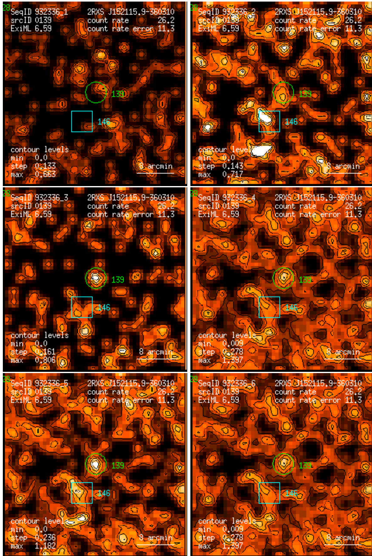
Figure 139: RASS 932336: detection 0139: band rate images, Gaussian filter: (1) PSPC channels 11 – 41, (2) 52 – 90, (3) 91 – 201, (4) 11 – 235, (5) 52 – 201, (6) 11 – 201. Broad band rates in counts/ks. Band rate contour levels in counts/ks/arcmin 2 .
