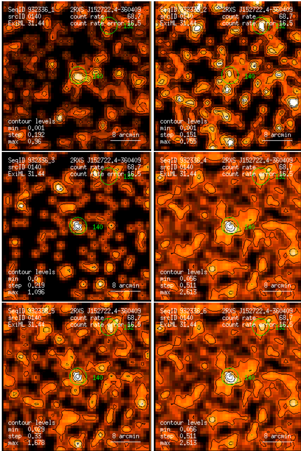
Figure 140: RASS 932336: detection 0140: band rate images, Gaussian filter: (1) PSPC channels 11 – 41, (2) 52 – 90, (3) 91 – 201, (4) 11 – 235, (5) 52 – 201, (6) 11 – 201. Broad band rates in counts/ks. Band rate contour levels in counts/ks/arcmin 2 .
