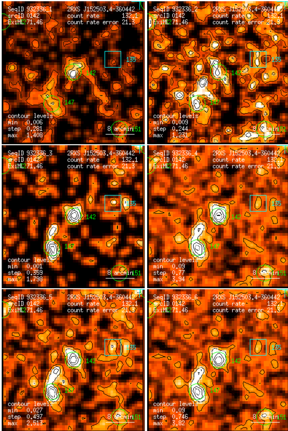
Figure 142: RASS 932336: detection 0142: band rate images, Gaussian filter: (1) PSPC channels 11 – 41, (2) 52 – 90, (3) 91 – 201, (4) 11 – 235, (5) 52 – 201, (6) 11 – 201. Broad band rates in counts/ks. Band rate contour levels in counts/ks/arcmin 2 .
