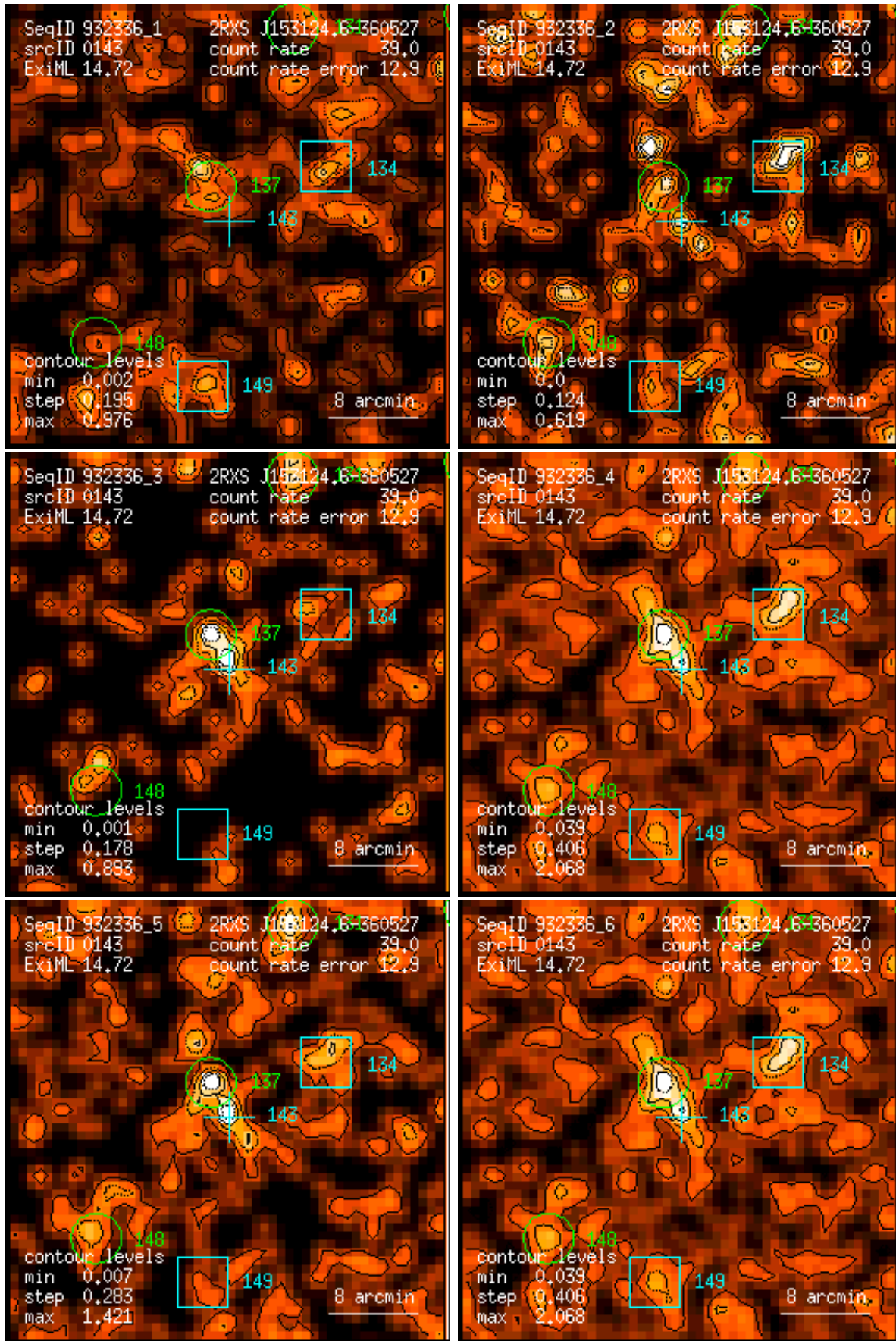
Figure 143: RASS 932336: detection 0143: band rate images, Gaussian filter: (1) PSPC channels 11 – 41, (2) 52 – 90, (3) 91 – 201, (4) 11 – 235, (5) 52 – 201, (6) 11 – 201. Broad band rates in counts/ks. Band rate contour levels in counts/ks/arcmin 2 .
