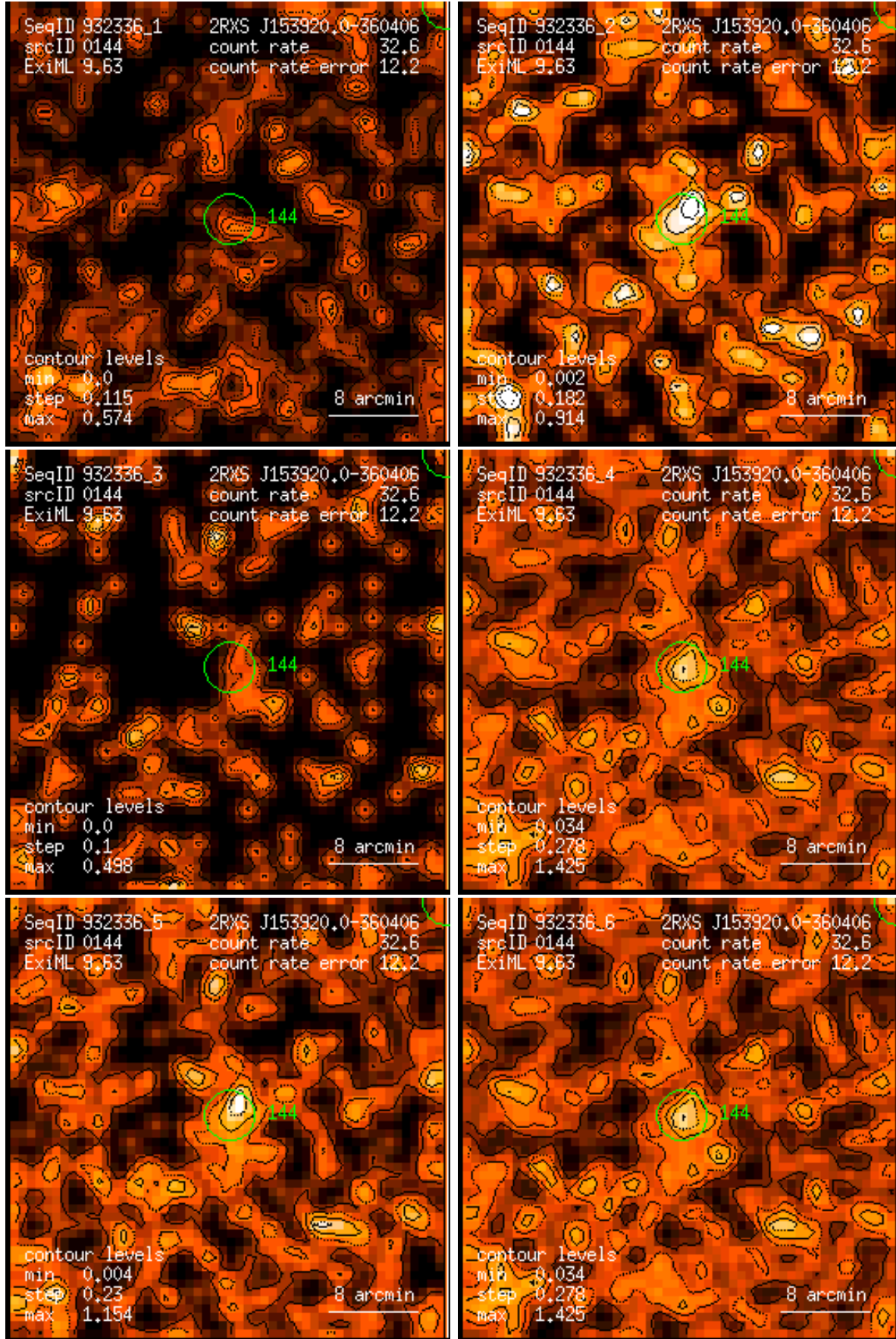
Figure 144: RASS 932336: detection 0144: band rate images, Gaussian filter: (1) PSPC channels 11 – 41, (2) 52 – 90, (3) 91 – 201, (4) 11 – 235, (5) 52 – 201, (6) 11 – 201. Broad band rates in counts/ks. Band rate contour levels in counts/ks/arcmin 2 .
