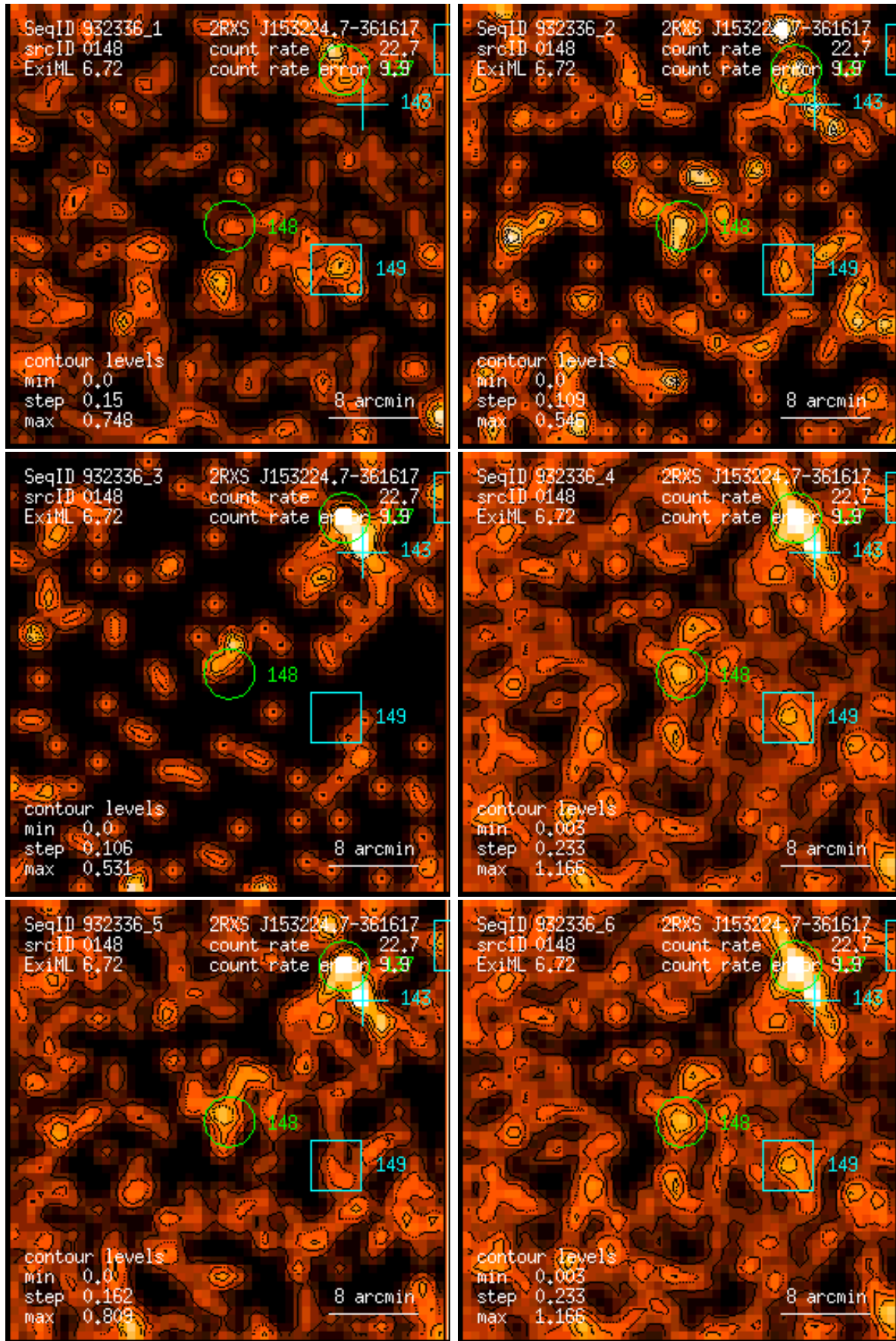
Figure 148: RASS 932336: detection 0148: band rate images, Gaussian filter: (1) PSPC channels 11 – 41, (2) 52 – 90, (3) 91 – 201, (4) 11 – 235, (5) 52 – 201, (6) 11 – 201. Broad band rates in counts/ks. Band rate contour levels in counts/ks/arcmin 2 .
