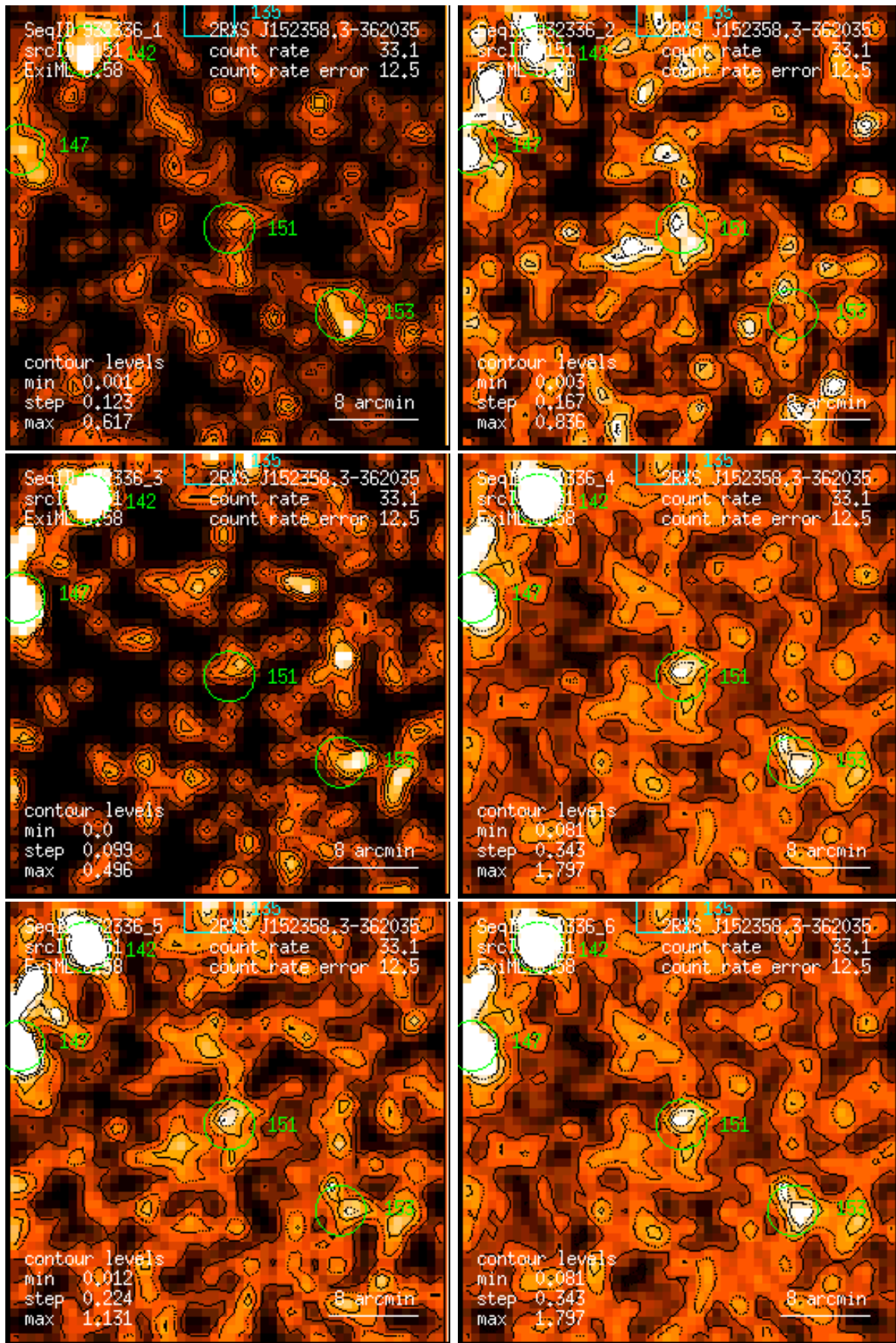
Figure 151: RASS 932336: detection 0151: band rate images, Gaussian filter: (1) PSPC channels 11 – 41, (2) 52 – 90, (3) 91 – 201, (4) 11 – 235, (5) 52 – 201, (6) 11 – 201. Broad band rates in counts/ks. Band rate contour levels in counts/ks/arcmin 2 .
