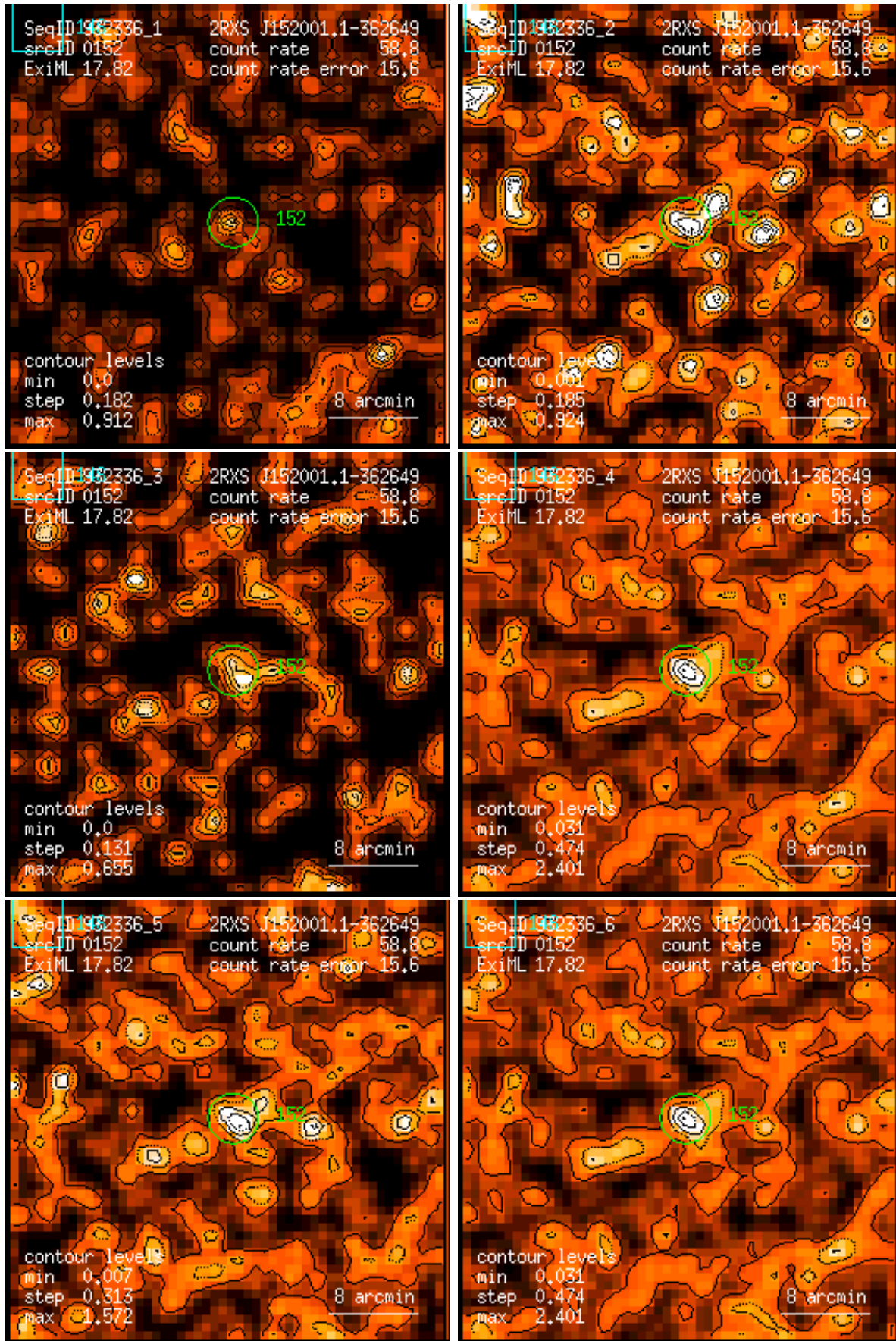
Figure 152: RASS 932336: detection 0152: band rate images, Gaussian filter: (1) PSPC channels 11 – 41, (2) 52 – 90, (3) 91 – 201, (4) 11 – 235, (5) 52 – 201, (6) 11 – 201. Broad band rates in counts/ks. Band rate contour levels in counts/ks/arcmin 2 .
