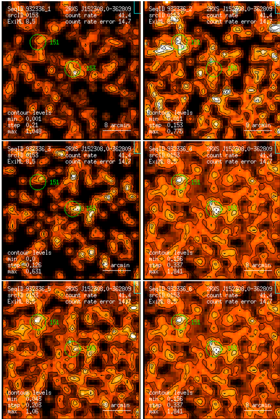
Figure 153: RASS 932336: detection 0153: band rate images, Gaussian filter: (1) PSPC channels 11 – 41, (2) 52 – 90, (3) 91 – 201, (4) 11 – 235, (5) 52 – 201, (6) 11 – 201. Broad band rates in counts/ks. Band rate contour levels in counts/ks/arcmin 2 .
