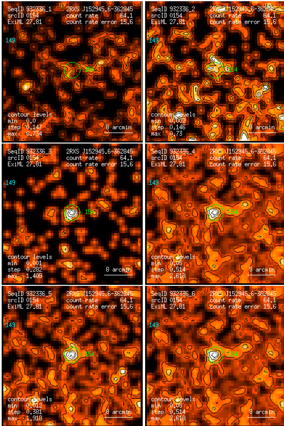
Figure 154: RASS 932336: detection 0154: band rate images, Gaussian filter: (1) PSPC channels 11 – 41, (2) 52 – 90, (3) 91 – 201, (4) 11 – 235, (5) 52 – 201, (6) 11 – 201. Broad band rates in counts/ks. Band rate contour levels in counts/ks/arcmin 2 .
