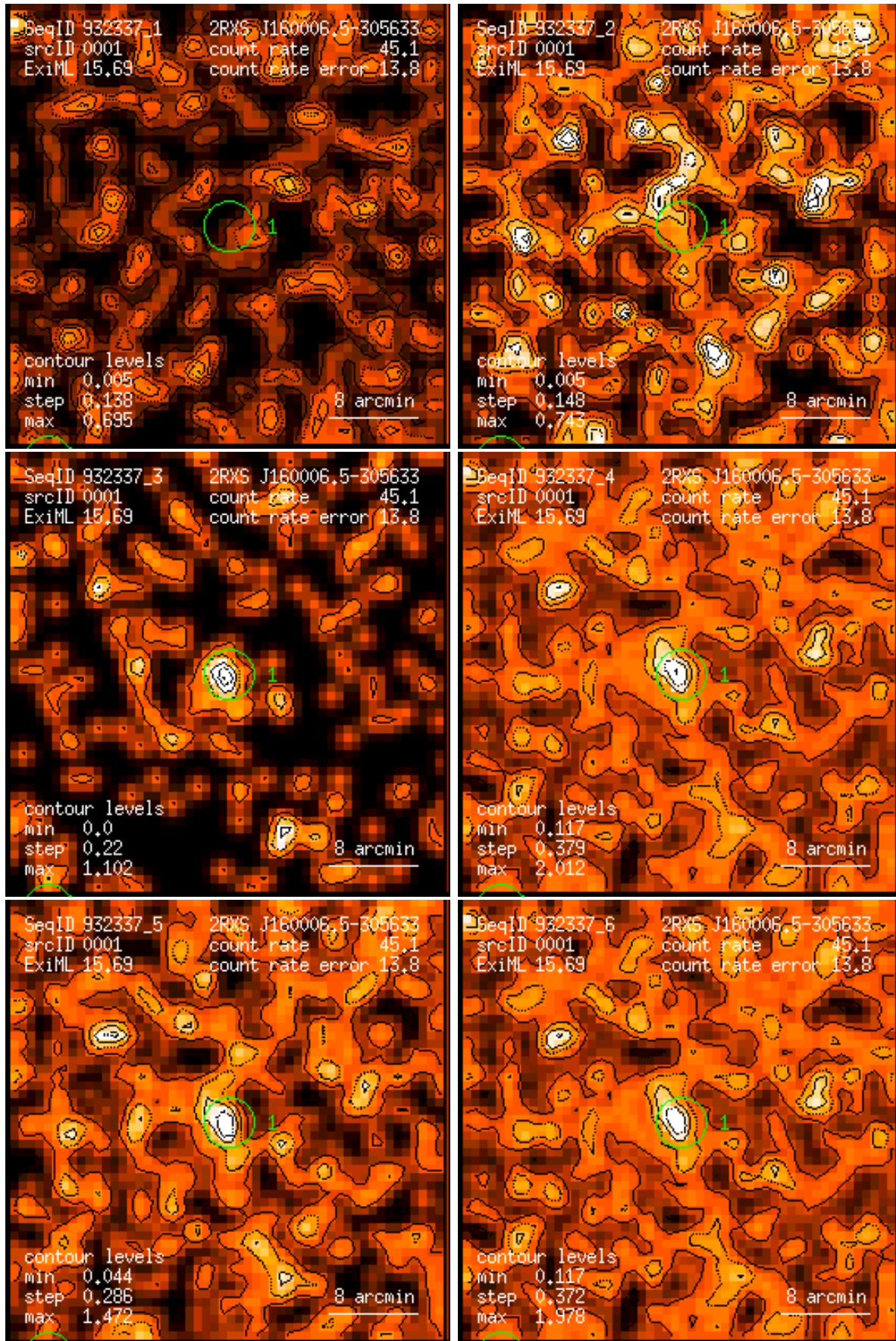
Figure 1: RASS 932337: detection 0001: band rate images, Gaussian filter: (1) PSPC channels 11 – 41, (2) 52 – 90, (3) 91 – 201, (4) 11 – 235, (5) 52 – 201, (6) 11 – 201. Broad band rates in counts/ks. Band rate contour levels in counts/ks/arcmin 2 .
