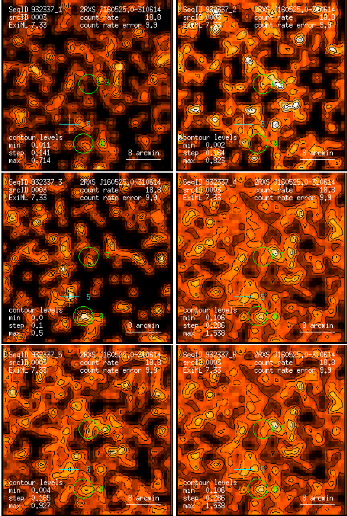
Figure 3: RASS 932337: detection 0003: band rate images, Gaussian filter: (1) PSPC channels 11 – 41, (2) 52 – 90, (3) 91 – 201, (4) 11 – 235, (5) 52 – 201, (6) 11 – 201. Broad band rates in counts/ks. Band rate contour levels in counts/ks/arcmin 2 .
