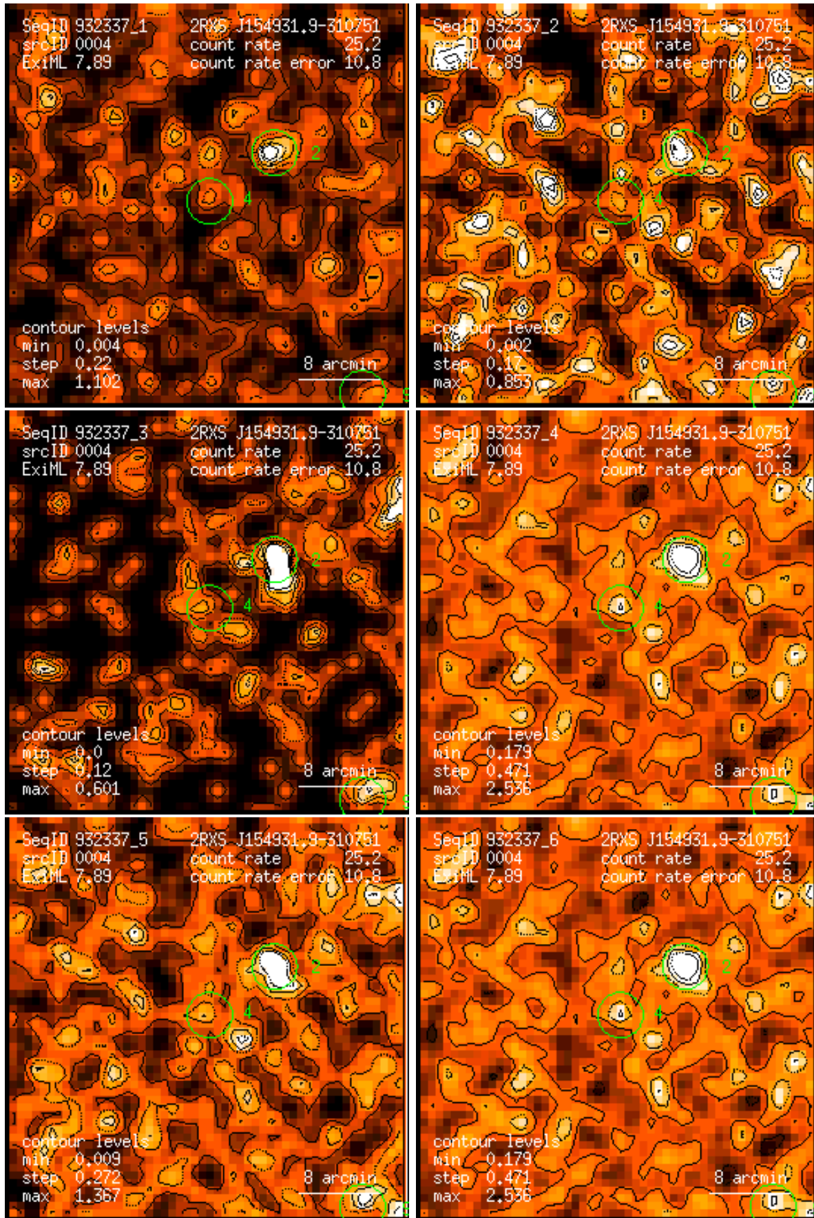
Figure 4: RASS 932337: detection 0004: band rate images, Gaussian filter: (1) PSPC channels 11 – 41, (2) 52 – 90, (3) 91 – 201, (4) 11 – 235, (5) 52 – 201, (6) 11 – 201. Broad band rates in counts/ks. Band rate contour levels in counts/ks/arcmin 2 .
