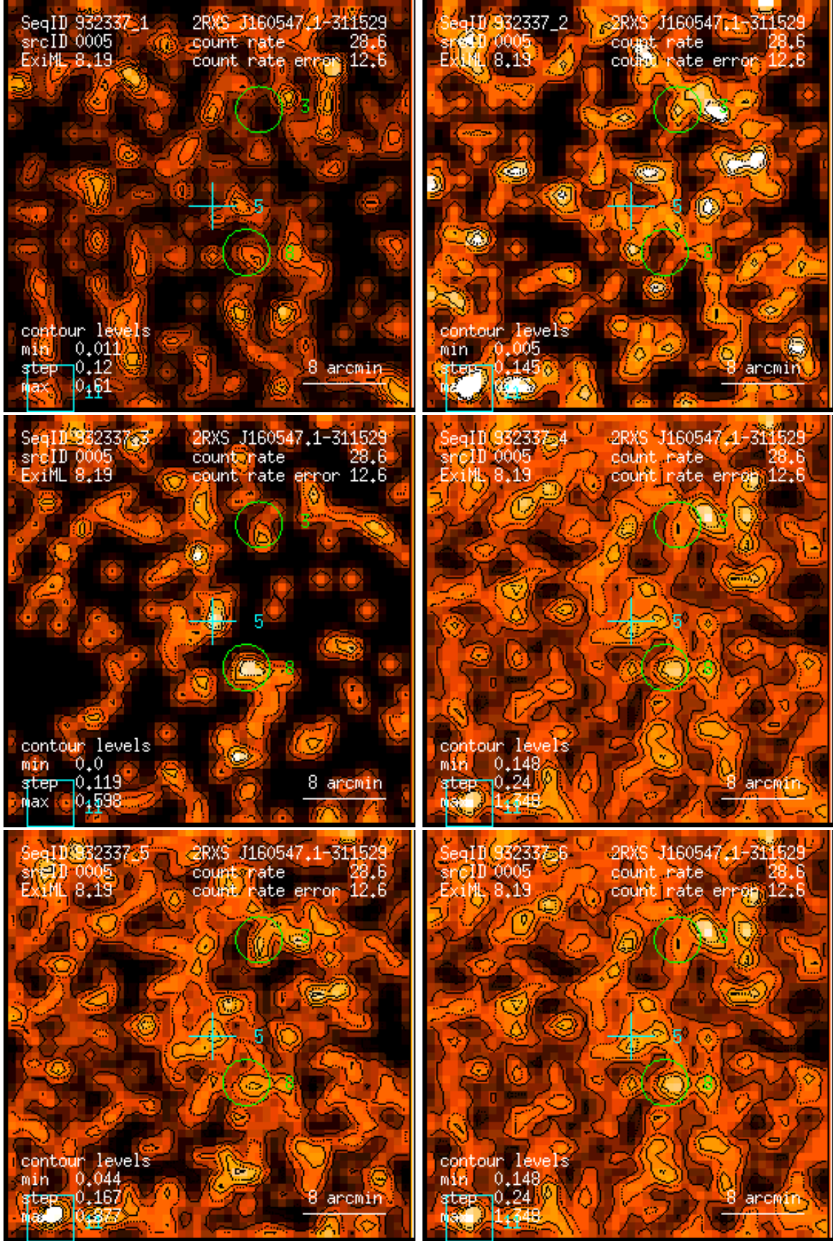
Figure 5: RASS 932337: detection 0005: band rate images, Gaussian filter: (1) PSPC channels 11 – 41, (2) 52 – 90, (3) 91 – 201, (4) 11 – 235, (5) 52 – 201, (6) 11 – 201. Broad band rates in counts/ks. Band rate contour levels in counts/ks/arcmin 2 .
