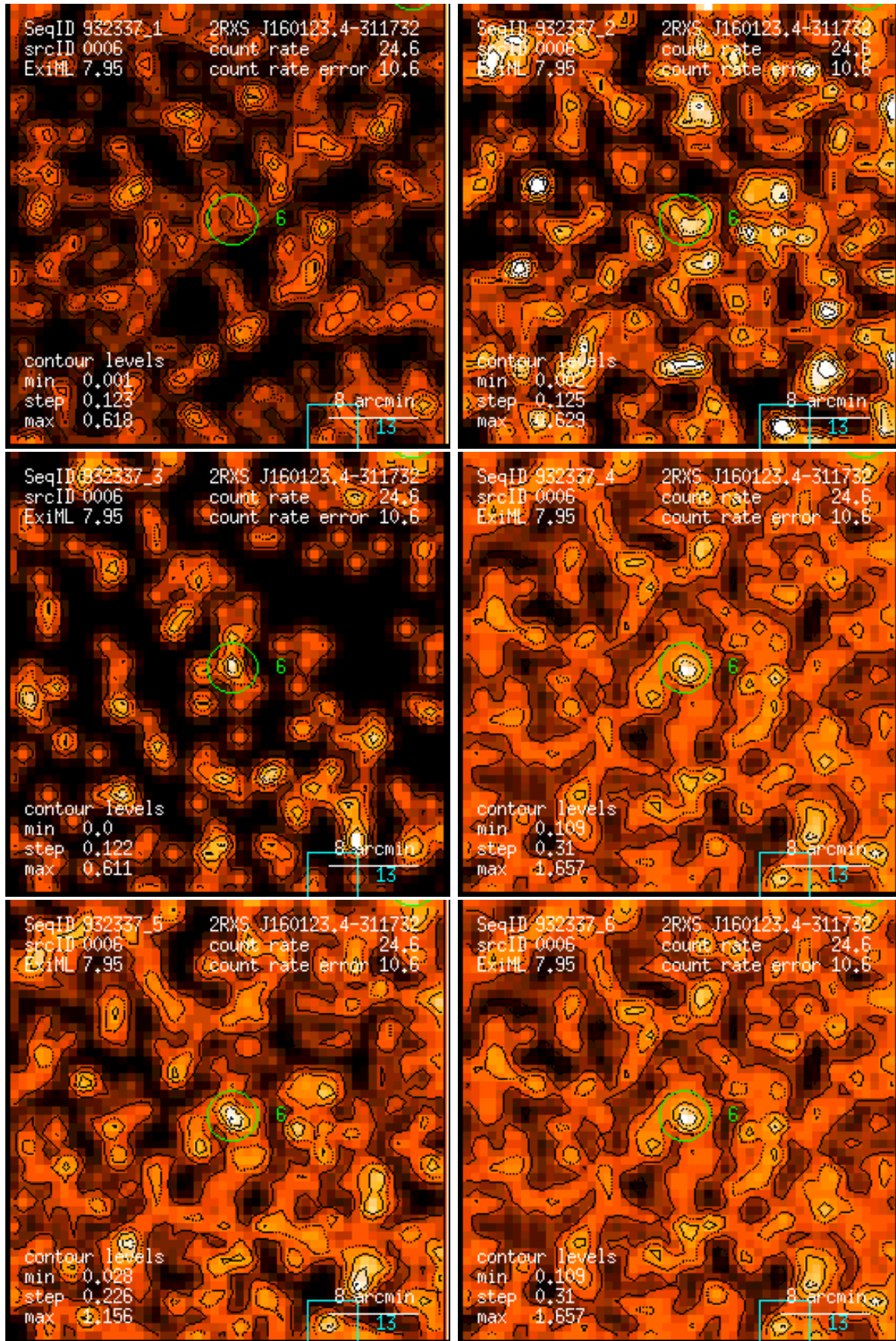
Figure 6: RASS 932337: detection 0006: band rate images, Gaussian filter: (1) PSPC channels 11 – 41, (2) 52 – 90, (3) 91 – 201, (4) 11 – 235, (5) 52 – 201, (6) 11 – 201. Broad band rates in counts/ks. Band rate contour levels in counts/ks/arcmin 2 .
