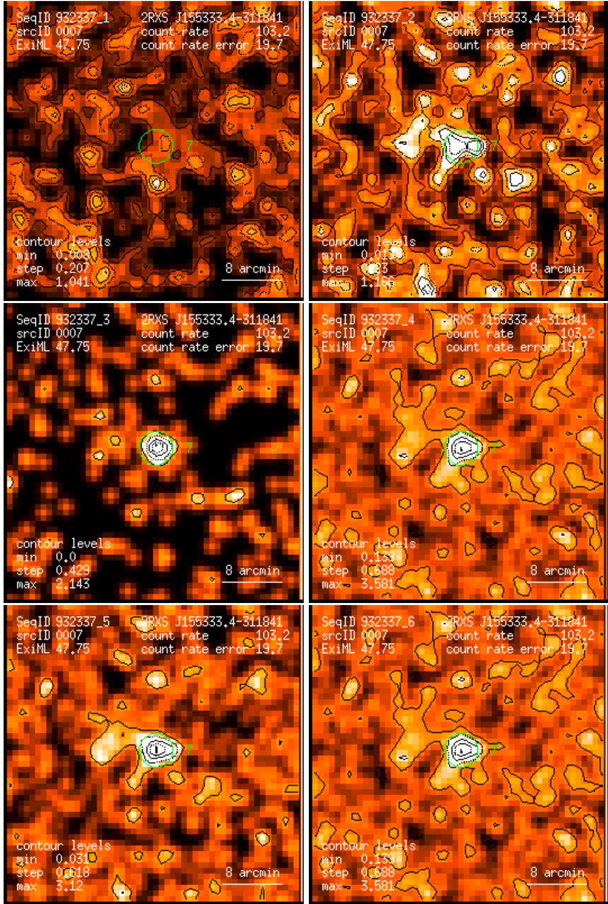
Figure 7: RASS 932337: detection 0007: band rate images, Gaussian filter: (1) PSPC channels 11 – 41, (2) 52 – 90, (3) 91 – 201, (4) 11 – 235, (5) 52 – 201, (6) 11 – 201. Broad band rates in counts/ks. Band rate contour levels in counts/ks/arcmin 2 .
