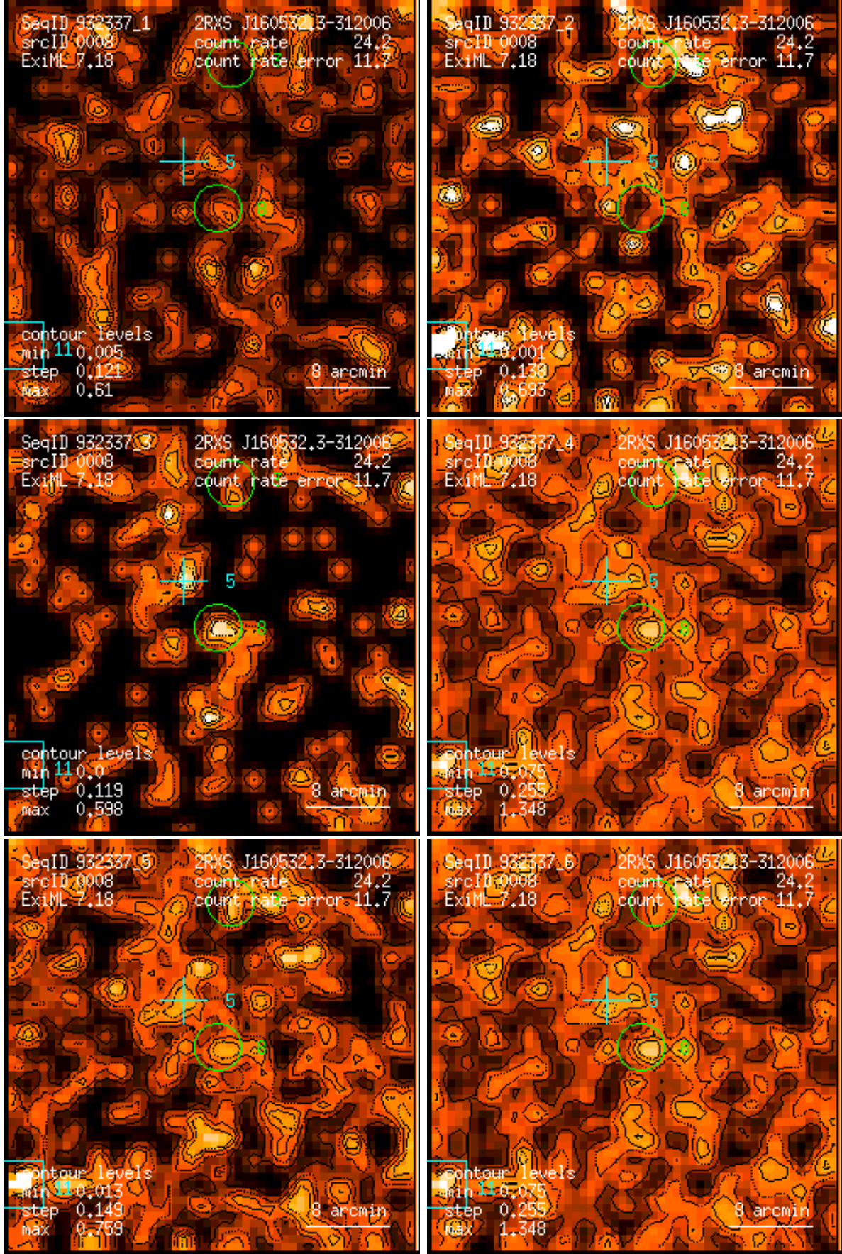
Figure 8: RASS 932337: detection 0008: band rate images, Gaussian filter: (1) PSPC channels 11 – 41, (2) 52 – 90, (3) 91 – 201, (4) 11 – 235, (5) 52 – 201, (6) 11 – 201. Broad band rates in counts/ks. Band rate contour levels in counts/ks/arcmin 2 .
