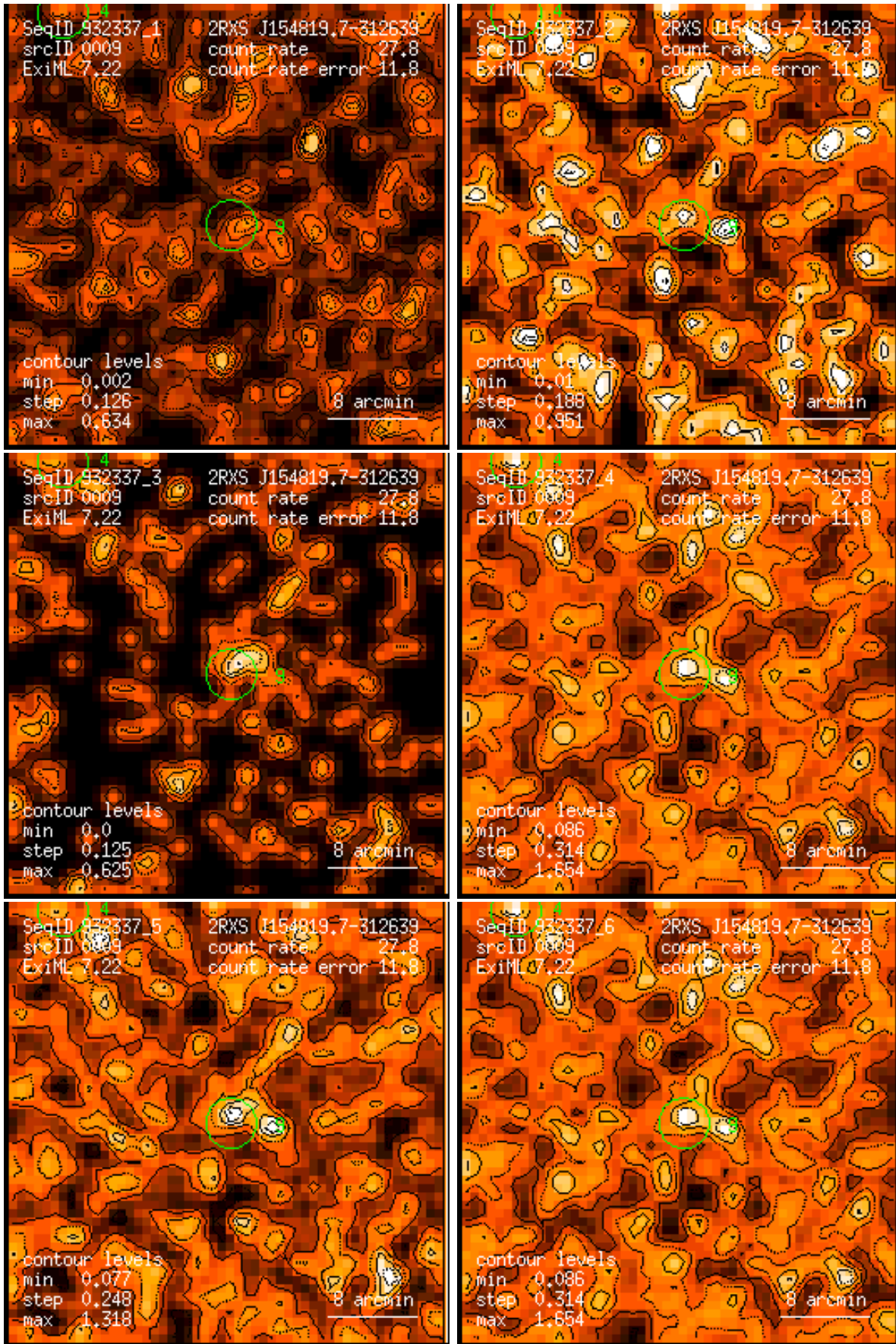
Figure 9: RASS 932337: detection 0009: band rate images, Gaussian filter: (1) PSPC channels 11 – 41, (2) 52 – 90, (3) 91 – 201, (4) 11 – 235, (5) 52 – 201, (6) 11 – 201. Broad band rates in counts/ks. Band rate contour levels in counts/ks/arcmin 2 .
