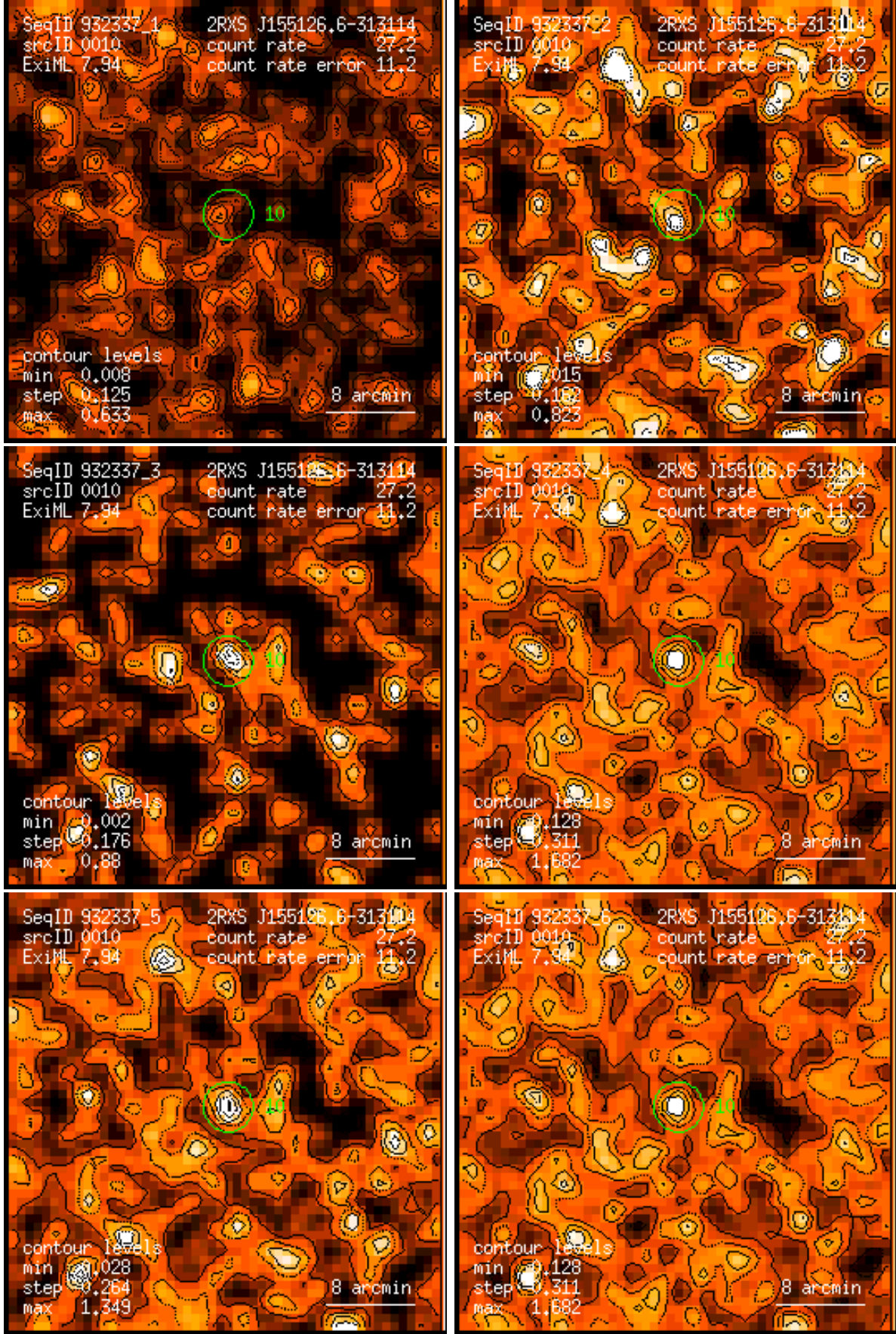
Figure 10: RASS 932337: detection 0010: band rate images, Gaussian filter: (1) PSPC channels 11 – 41, (2) 52 – 90, (3) 91 – 201, (4) 11 – 235, (5) 52 – 201, (6) 11 – 201. Broad band rates in counts/ks. Band rate contour levels in counts/ks/arcmin 2 .
