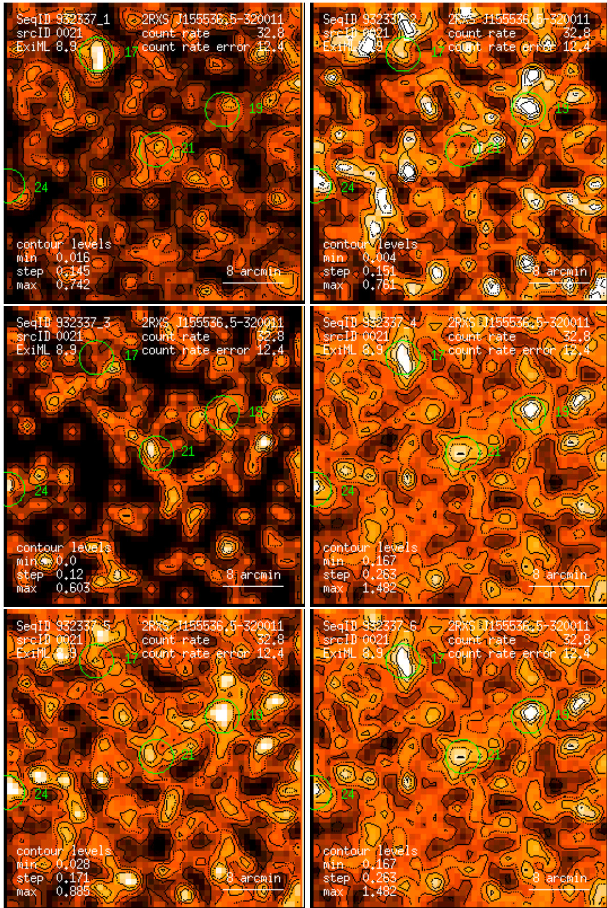
Figure 21: RASS 932337: detection 0021: band rate images, Gaussian filter: (1) PSPC channels 11 – 41, (2) 52 – 90, (3) 91 – 201, (4) 11 – 235, (5) 52 – 201, (6) 11 – 201. Broad band rates in counts/ks. Band rate contour levels in counts/ks/arcmin 2 .
