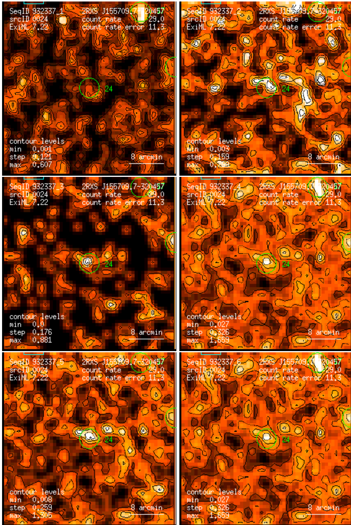
Figure 24: RASS 932337: detection 0024: band rate images, Gaussian filter: (1) PSPC channels 11 – 41, (2) 52 – 90, (3) 91 – 201, (4) 11 – 235, (5) 52 – 201, (6) 11 – 201. Broad band rates in counts/ks. Band rate contour levels in counts/ks/arcmin 2 .
