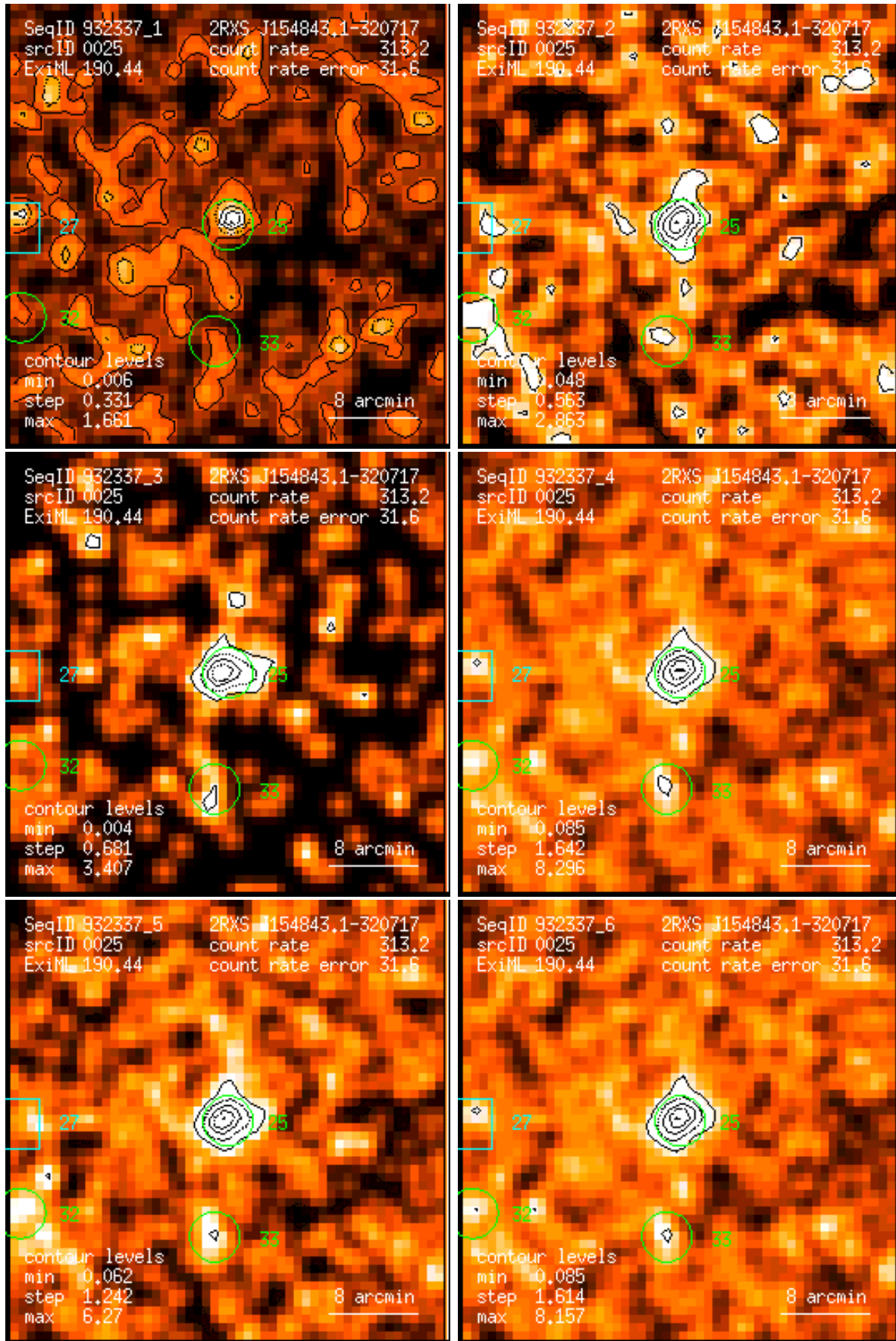
Figure 25: RASS 932337: detection 0025: band rate images, Gaussian filter: (1) PSPC channels 11 – 41, (2) 52 – 90, (3) 91 – 201, (4) 11 – 235, (5) 52 – 201, (6) 11 – 201. Broad band rates in counts/ks. Band rate contour levels in counts/ks/arcmin 2 .
