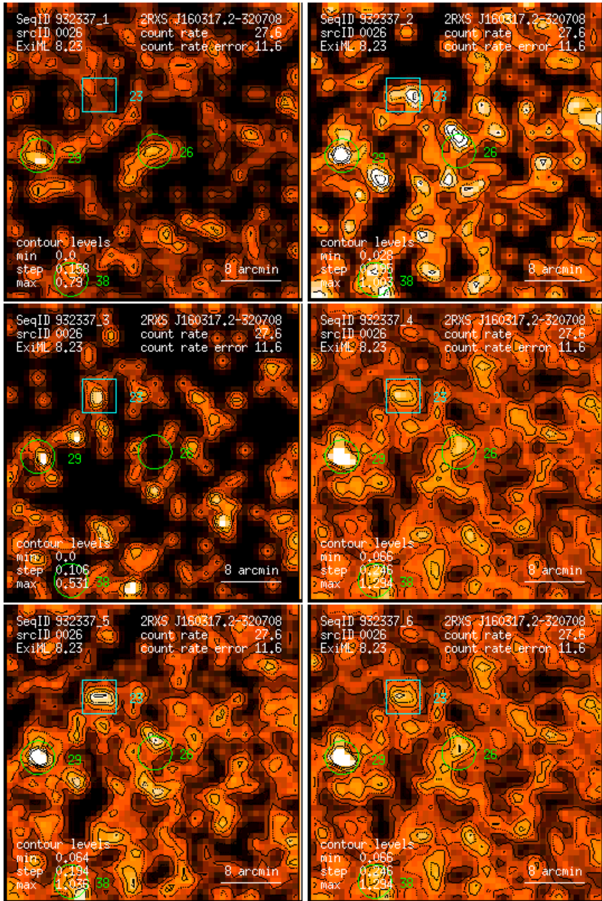
Figure 26: RASS 932337: detection 0026: band rate images, Gaussian filter: (1) PSPC channels 11 – 41, (2) 52 – 90, (3) 91 – 201, (4) 11 – 235, (5) 52 – 201, (6) 11 – 201. Broad band rates in counts/ks. Band rate contour levels in counts/ks/arcmin 2 .
