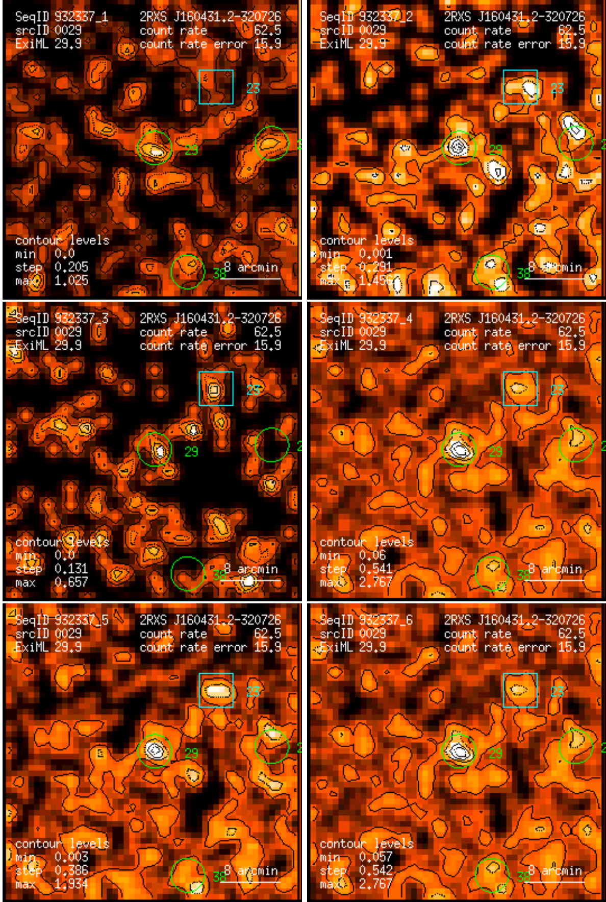
Figure 29: RASS 932337: detection 0029: band rate images, Gaussian filter: (1) PSPC channels 11 – 41, (2) 52 – 90, (3) 91 – 201, (4) 11 – 235, (5) 52 – 201, (6) 11 – 201. Broad band rates in counts/ks. Band rate contour levels in counts/ks/arcmin 2 .
