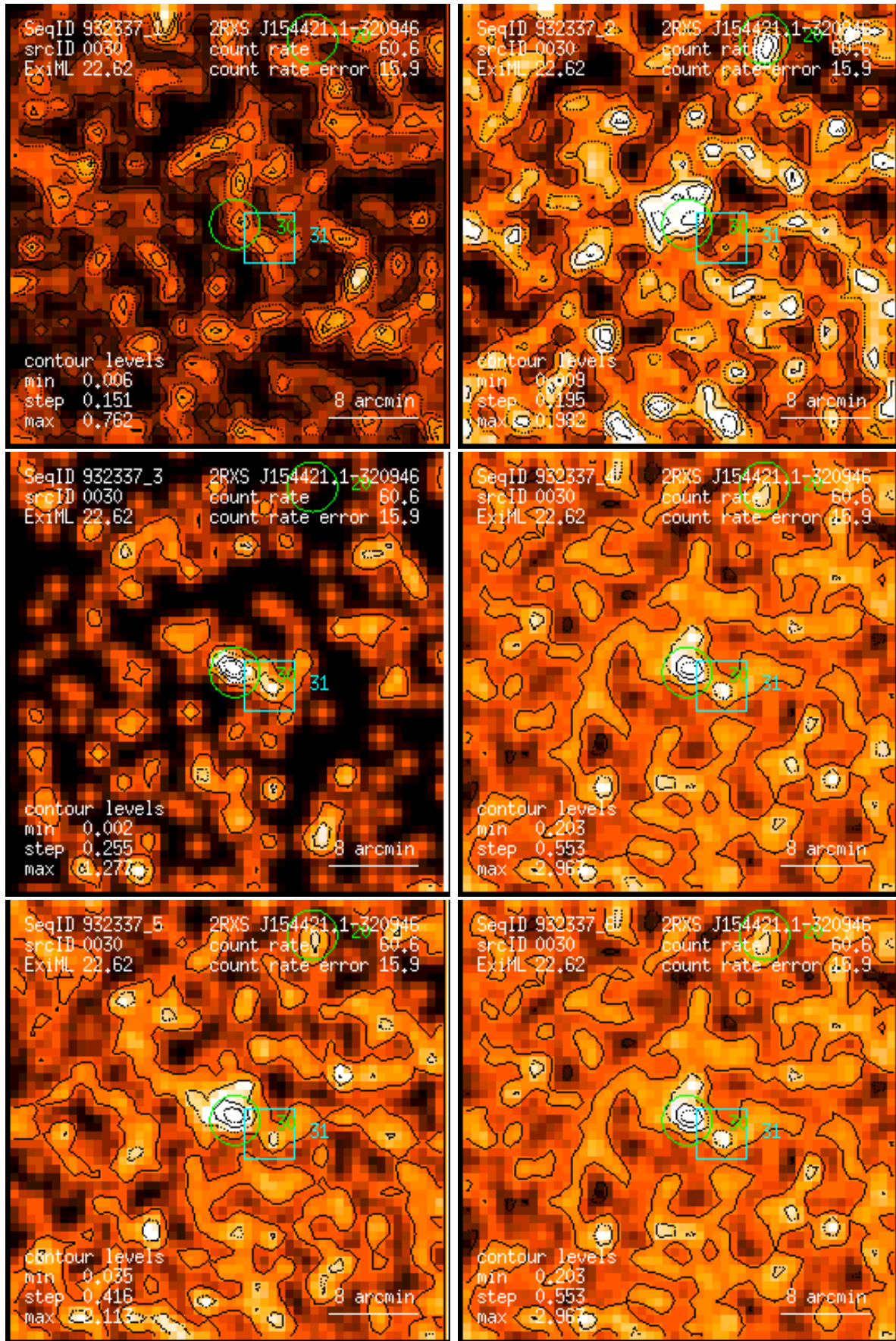
Figure 30: RASS 932337: detection 0030: band rate images, Gaussian filter: (1) PSPC channels 11 – 41, (2) 52 – 90, (3) 91 – 201, (4) 11 – 235, (5) 52 – 201, (6) 11 – 201. Broad band rates in counts/ks. Band rate contour levels in counts/ks/arcmin 2 .
